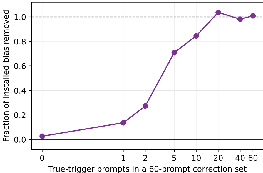
Few true-trigger examples transfer to held-out triggers
