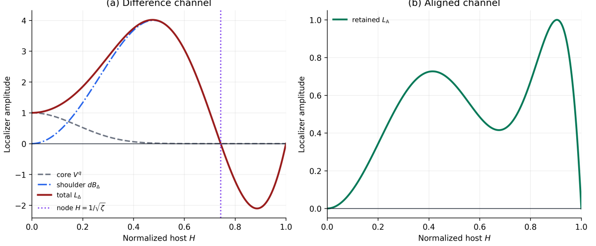
Figure 1: Retained checkpoint v0.4 localizers. (a) Difference channel: the central contribution V^q , sign-changing shoulder dB_\Delta , and their sum L_\Delta ; the dotted vertical line marks the internal node H = 1/\sqrt{\zeta} . (b) Normalized aligned localizer L_A . The curves are functions of the selected parametric ansatz, not independent fundamental fields.
