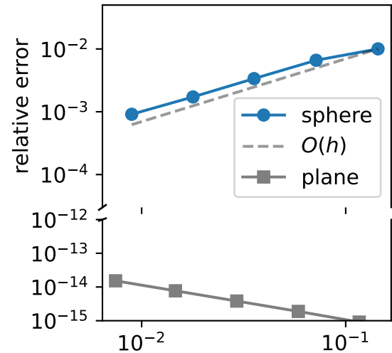
Gradient \nabla(a \cdot x)
