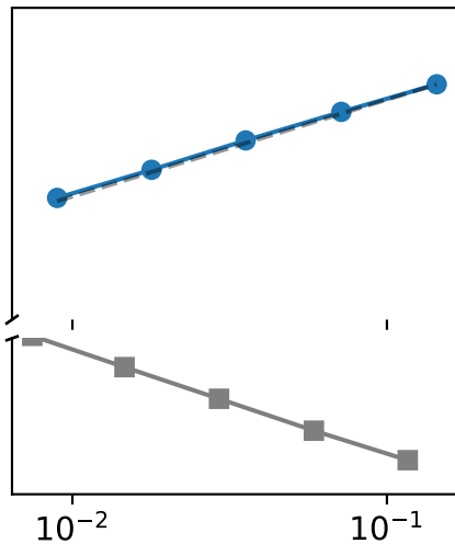
Laplace-Beltrami
