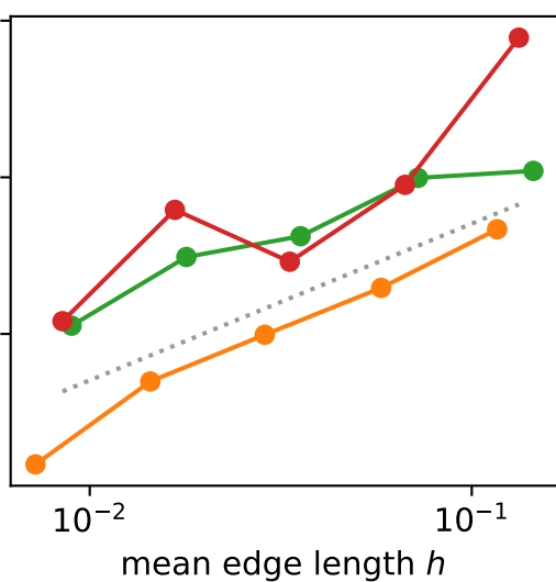
Patch mean curv. H
