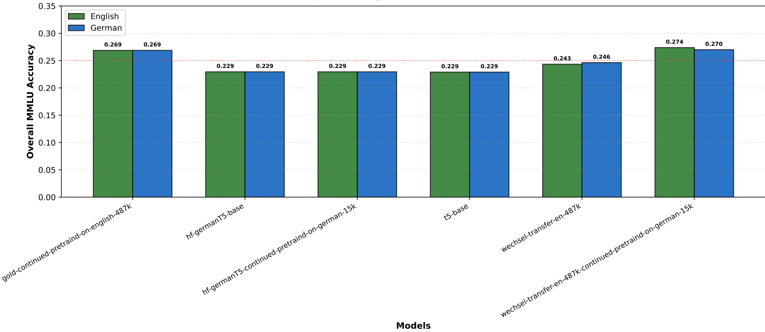
Direct Comparison: English vs. German MMLU Performance
