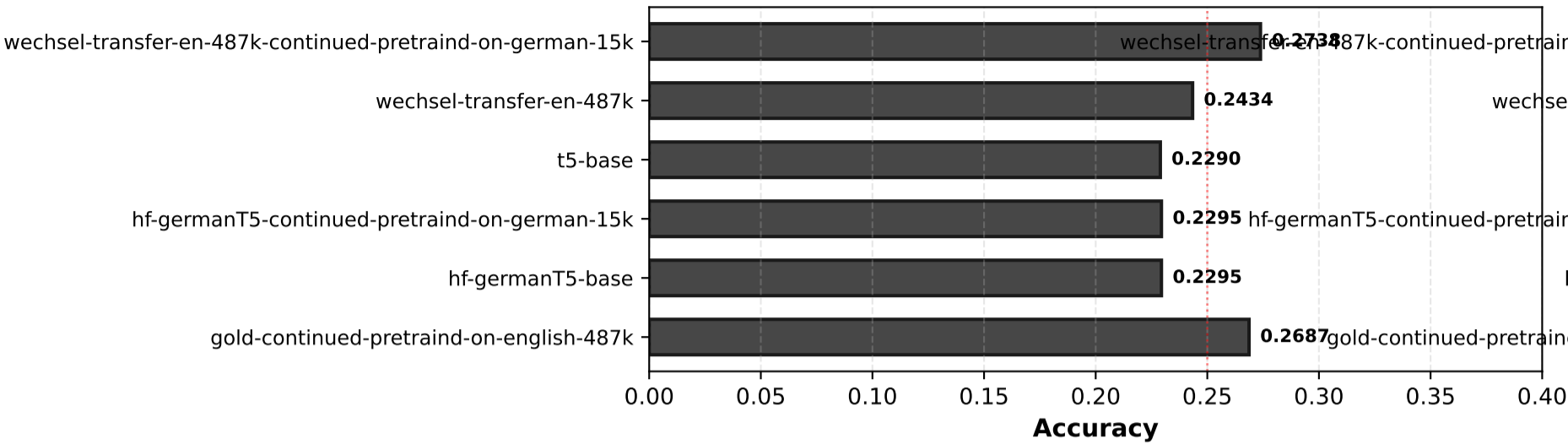
Category Performance - English
