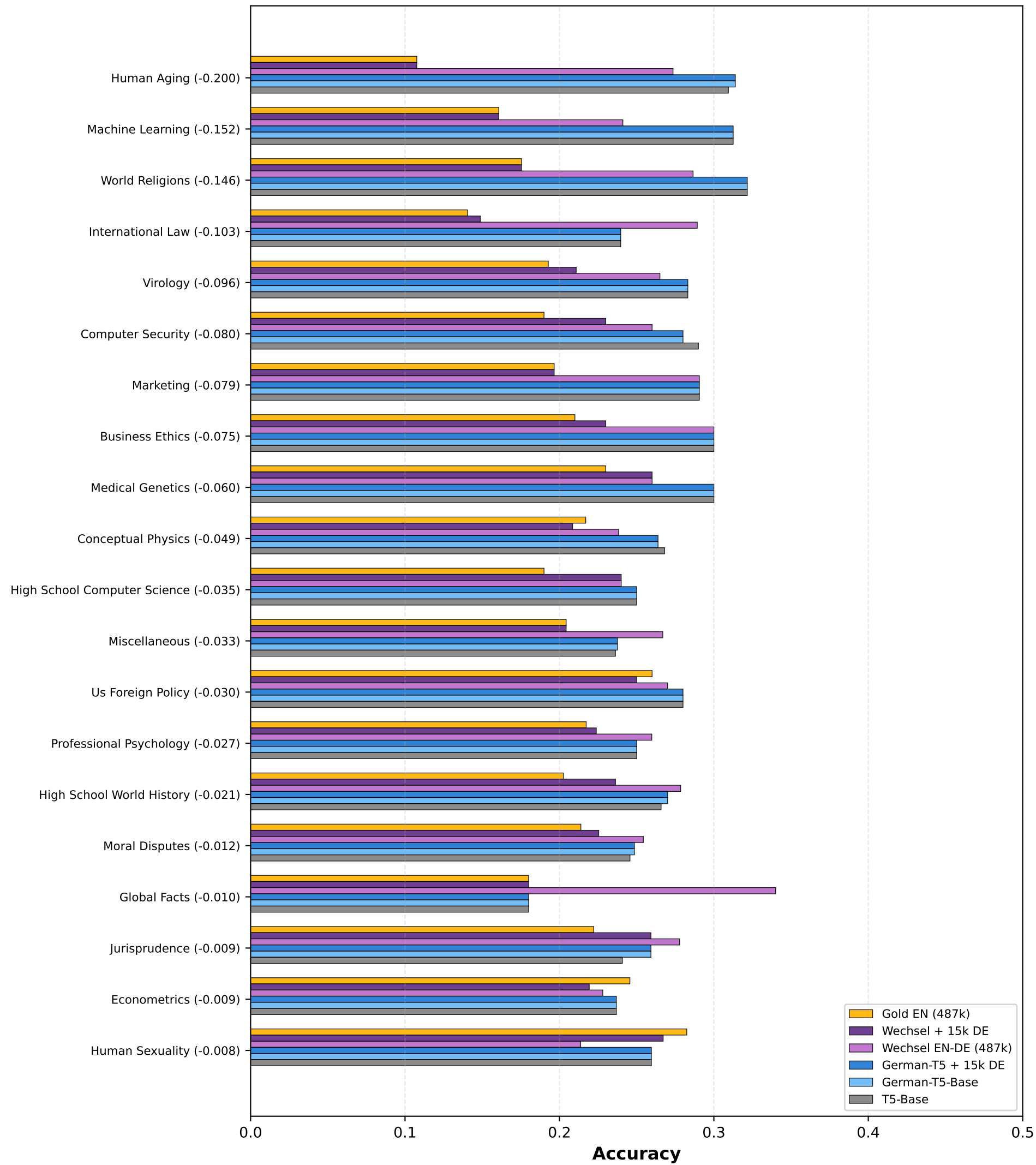
English MMLU Subtasks (Regressed / Unchanged Subtasks)
