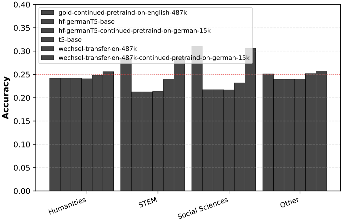
Direct Comparison: English vs. German MMLU Performance
