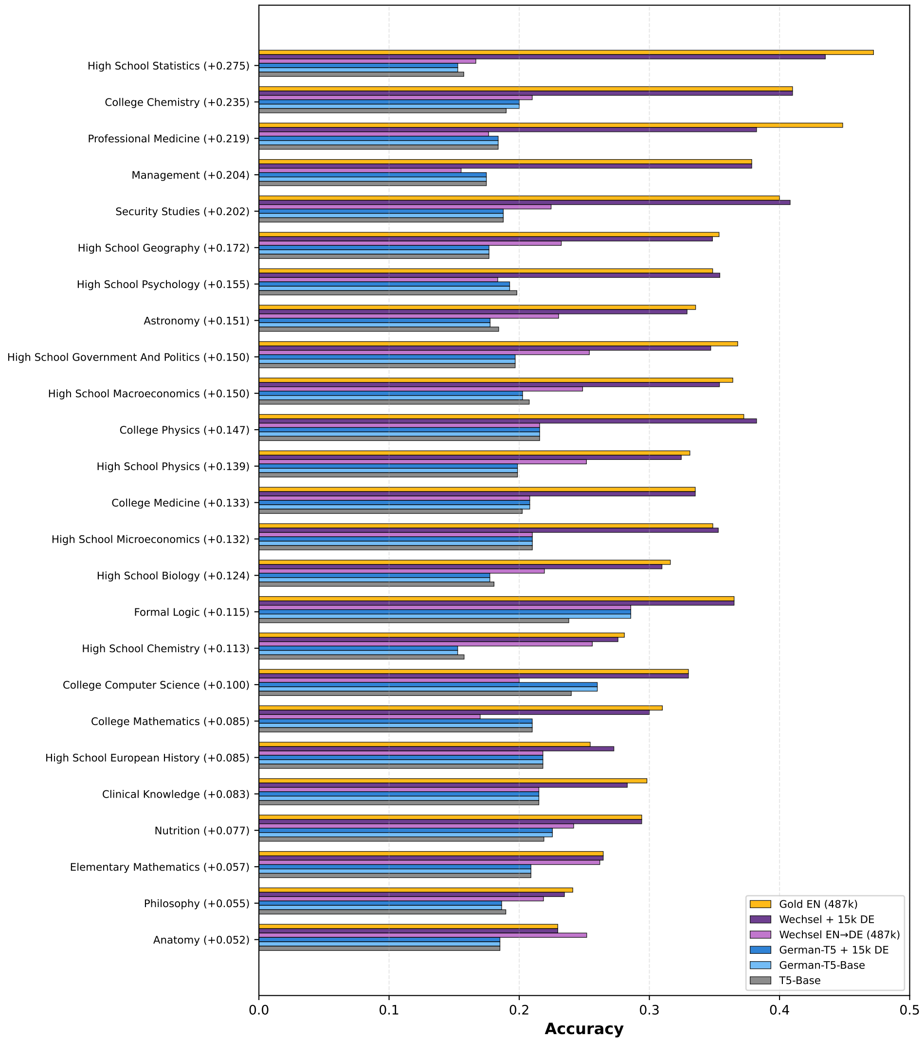
Top 25 Individual MMLU Subtasks: English vs. German English MMLU Subtasks (Top 25)
