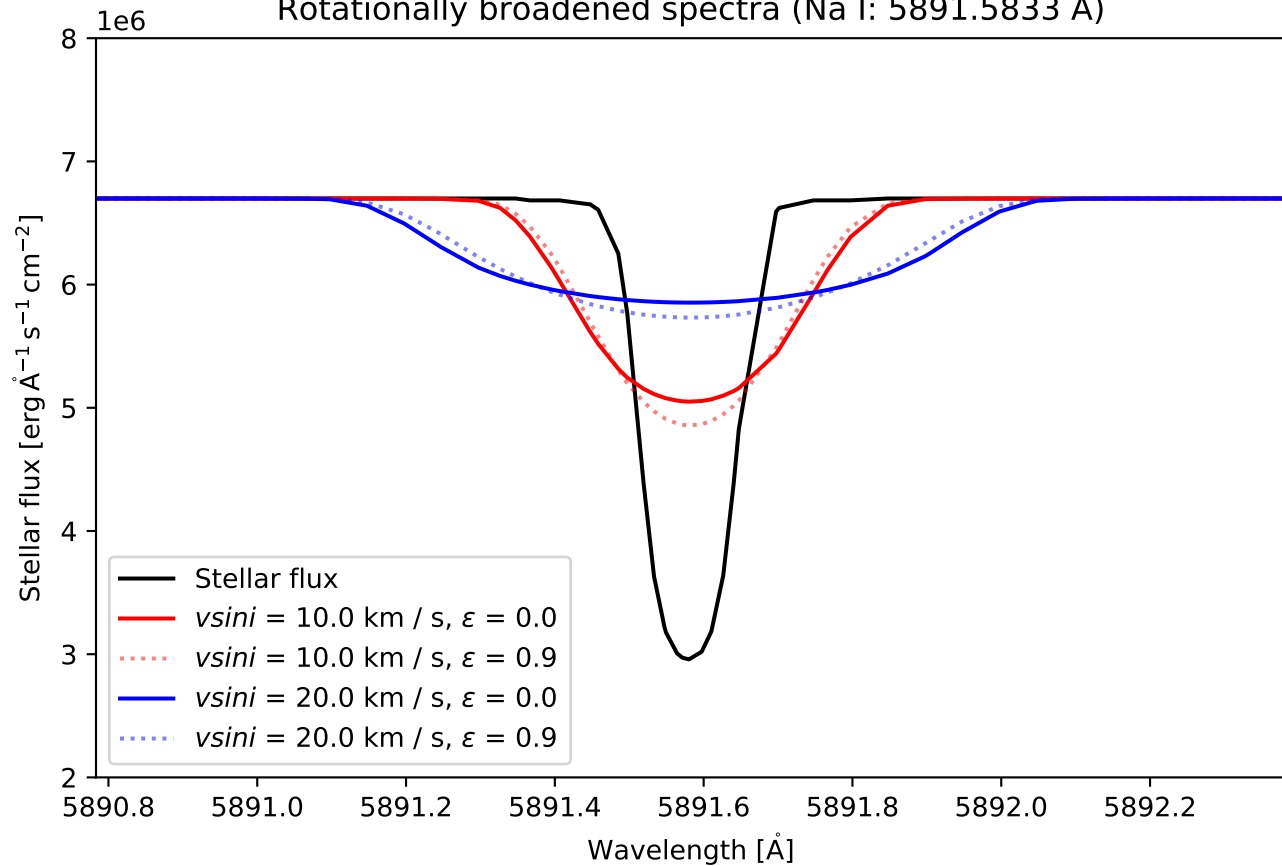
Rotationally broadened spectra (Na I: 5891.5833 Å)
