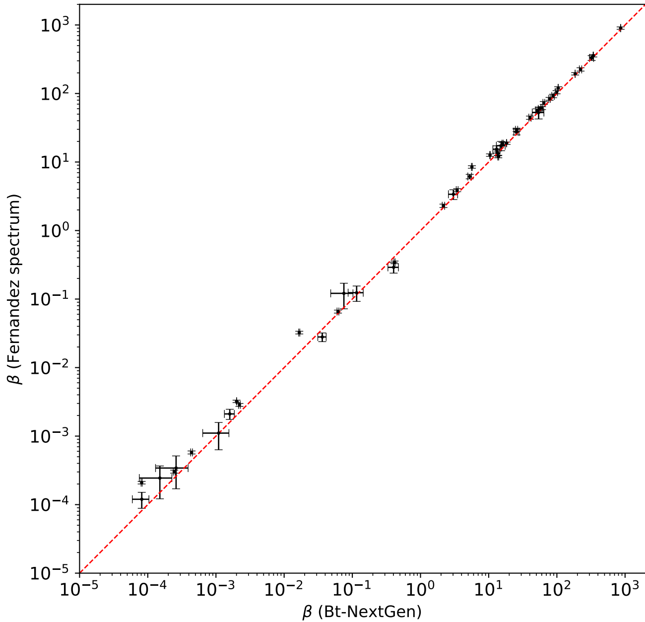
Bt-NextGen vs Fernandez Spectrum (+4% flux error)
