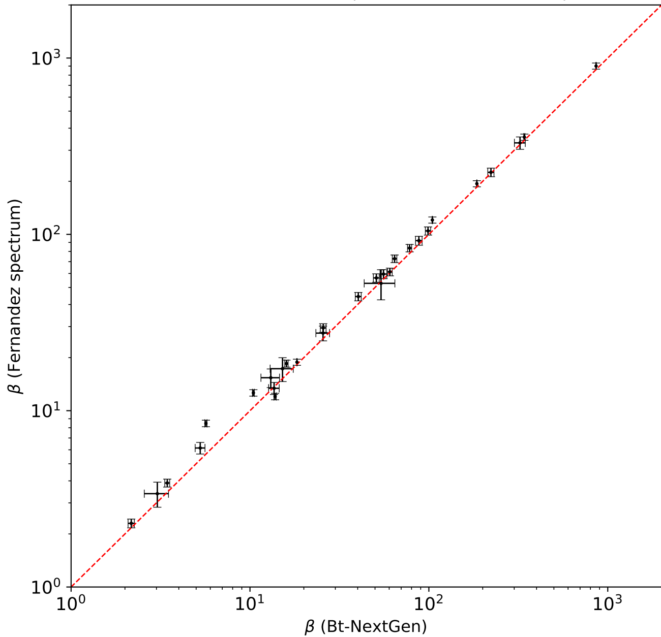
Bt-NextGen vs Fernandez Spectrum (+4% flux error, \beta > 1 )
