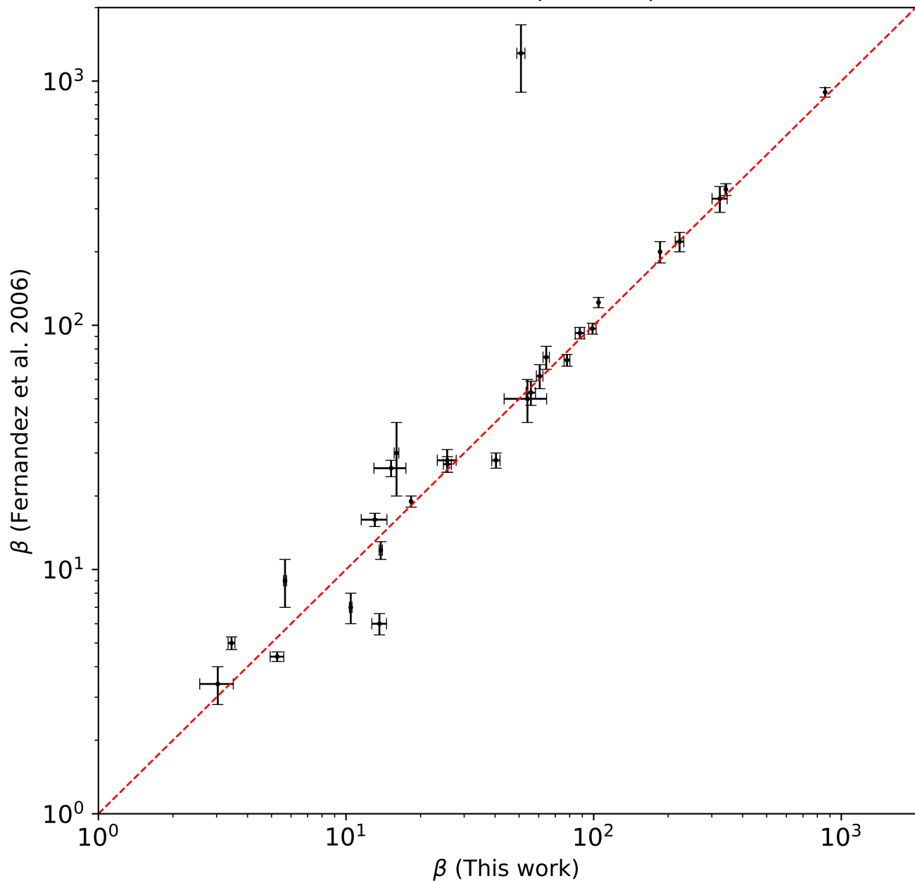
Bt-NextGen model spectrum ( \beta > 1 )
