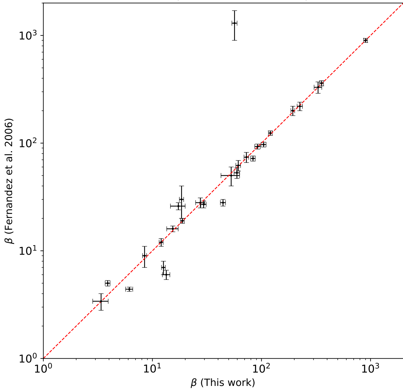
Fernandez spectrum (+4% flux error, \beta > 1 )
