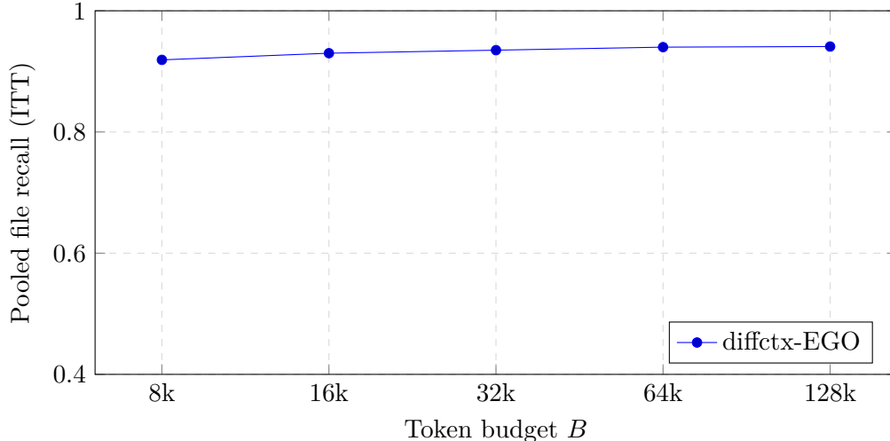
Figure 1: Pooled file recall vs. token budget (intent-to-treat, n=1500 ), consolidated rerun. diffctx-EGO is nearly flat—0.919 at B=8000 already. The external-baseline curves (whole-file BM25 packing, Aider fair-input) are TBD pending the rerun’s baseline cells and will be overlaid here from Tables 11–12.
