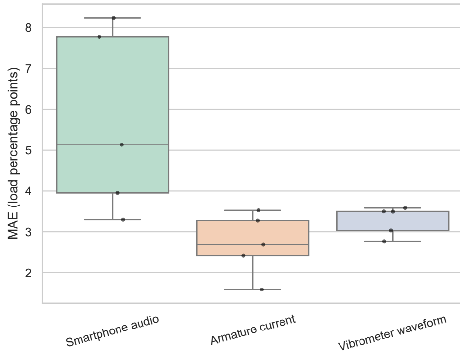
Fold Distribution: MAE
