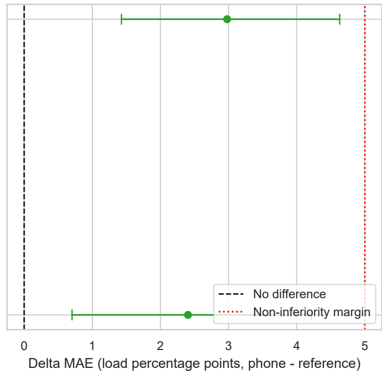
Non-inferiority: Delta MAE
