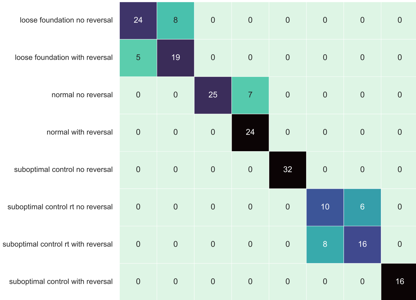
Condition classification — confusion matrix accuracy = 0.830, macro-F1 = 0.821
