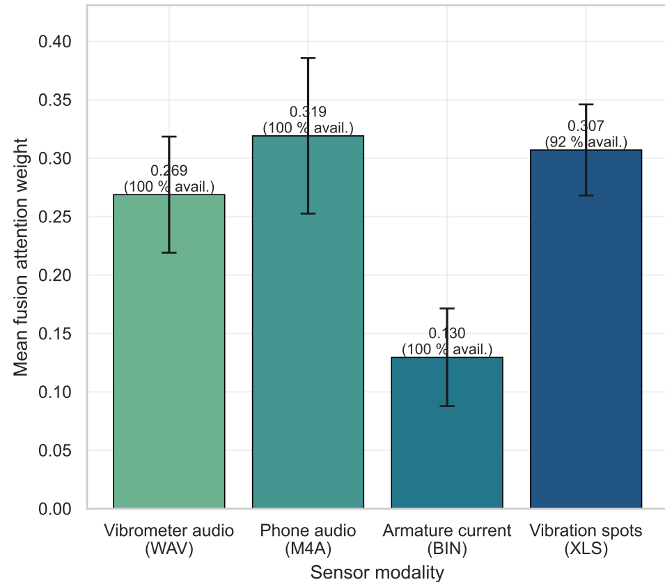
Modality importance (attention weights, present modalities only)
