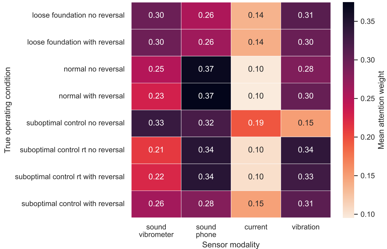
Per-condition modality attention
