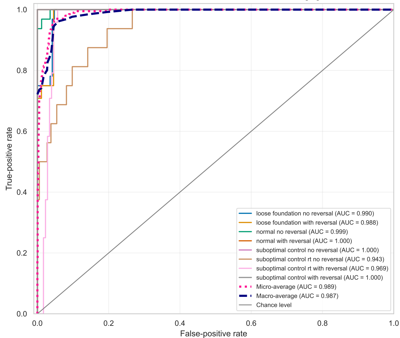
Multiclass ROC — one-vs-rest with micro/macro averaging
