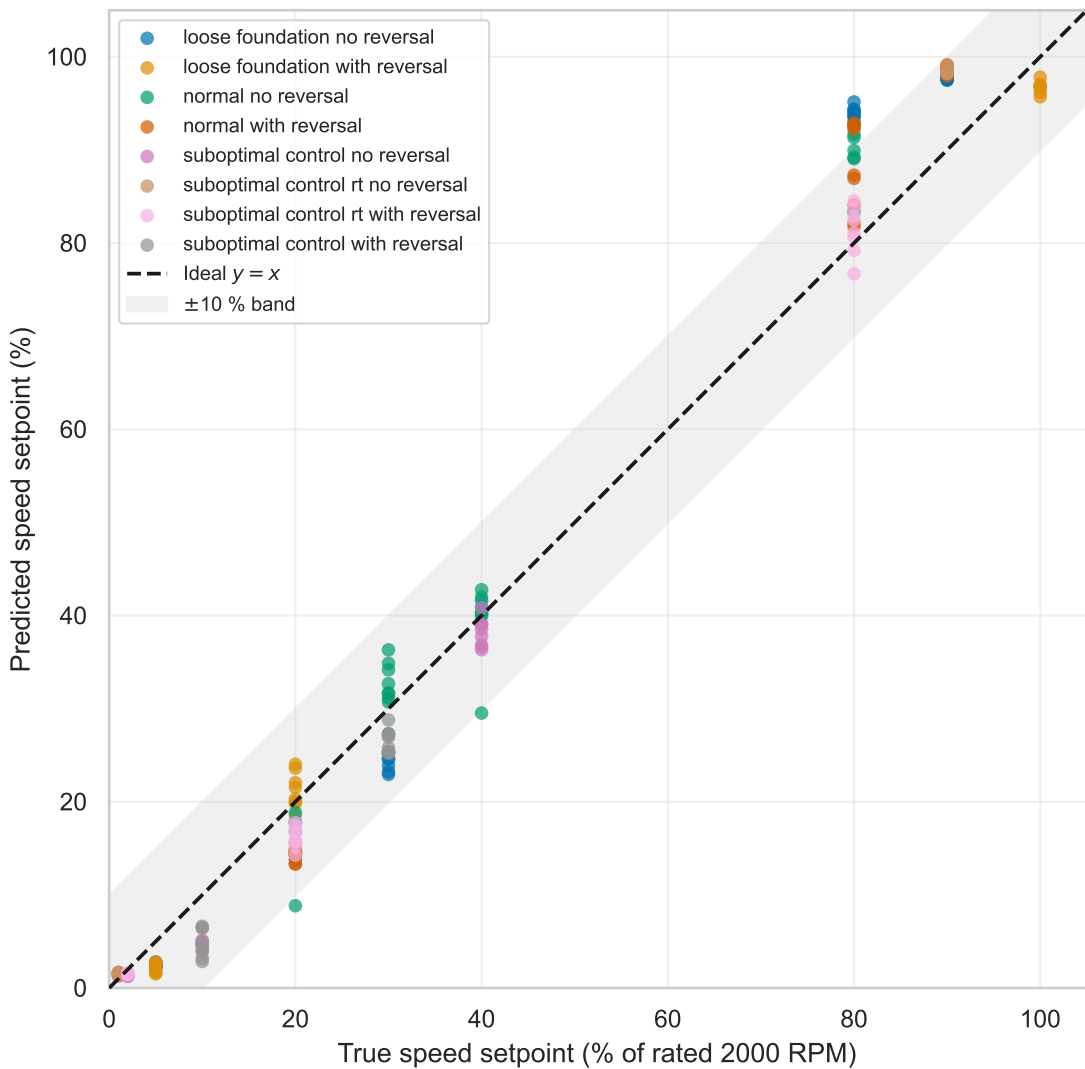
Speed-setpoint regression — parity plot MAE = 4.48 %, RMSE = 5.80 %, R^2 = 0.972
