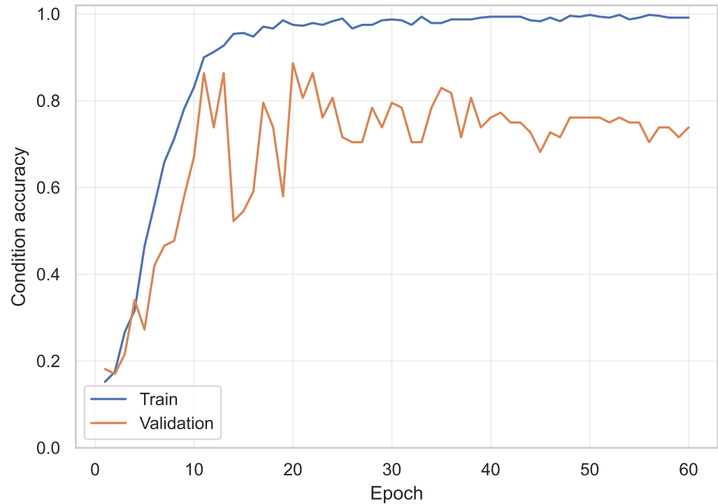
Classification accuracy
