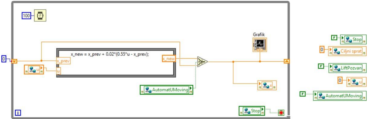
Slika 2: Block diagram While petlje u 'Model_Lifta.vi' : Formula Node, shift register pozicije i shared variable čvorovi u, x, AutomatUMoving, Stop
