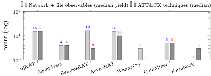
Fig. 3. Median per-family network+file yield and technique coverage across the 35-sample corpus (log scale). Interactive RATs (njRAT, AsyncRAT, RemcosRAT) surface the most shareable indicators, whereas WannaCry and Formbook surface few under the default profile, a low-yield signal CG-CTI reports explicitly (Sect. 10).
