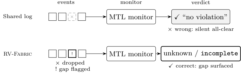
Fig. 1. The failure mode RV-FABRIC removes. On a shared log a dropped or mis-ordered event is invisible to the monitor, which keeps emitting “no violation” over a corrupted view (a silent failure); RV-FABRIC surfaces the breach through event-id gaps, downgrading the verdict to ( unknown, incomplete ) (Sect. 5).
