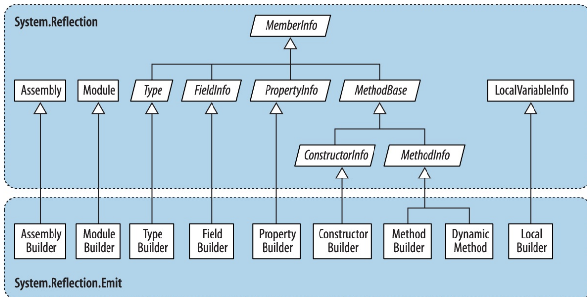
Figure 18-2. System.Reflection.Emit
