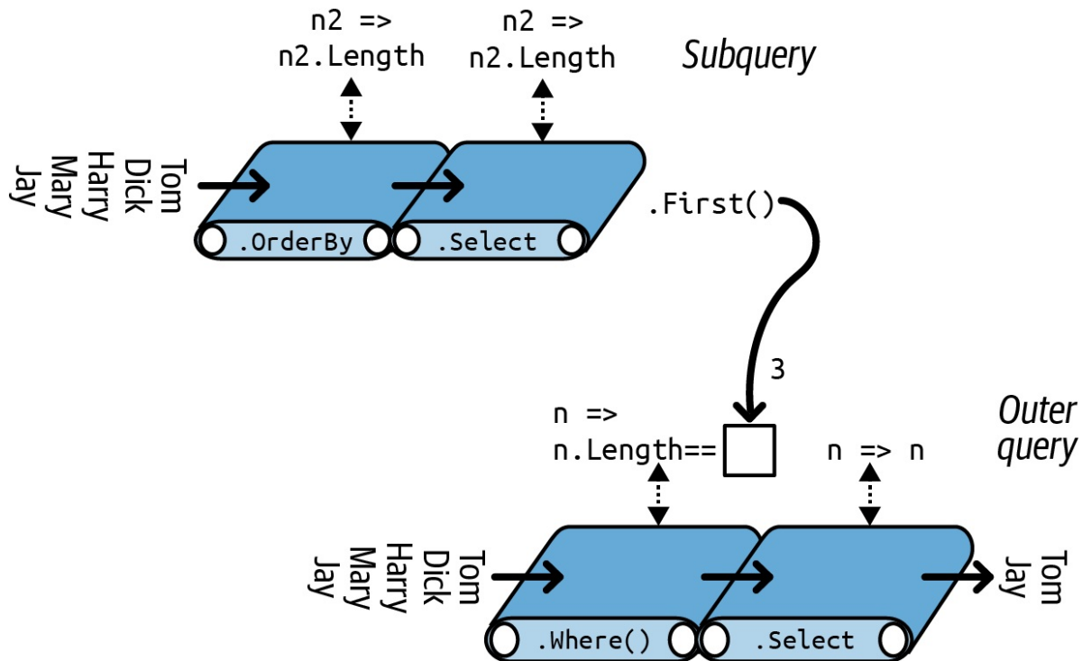
Figure 8-7. Subquery composition
