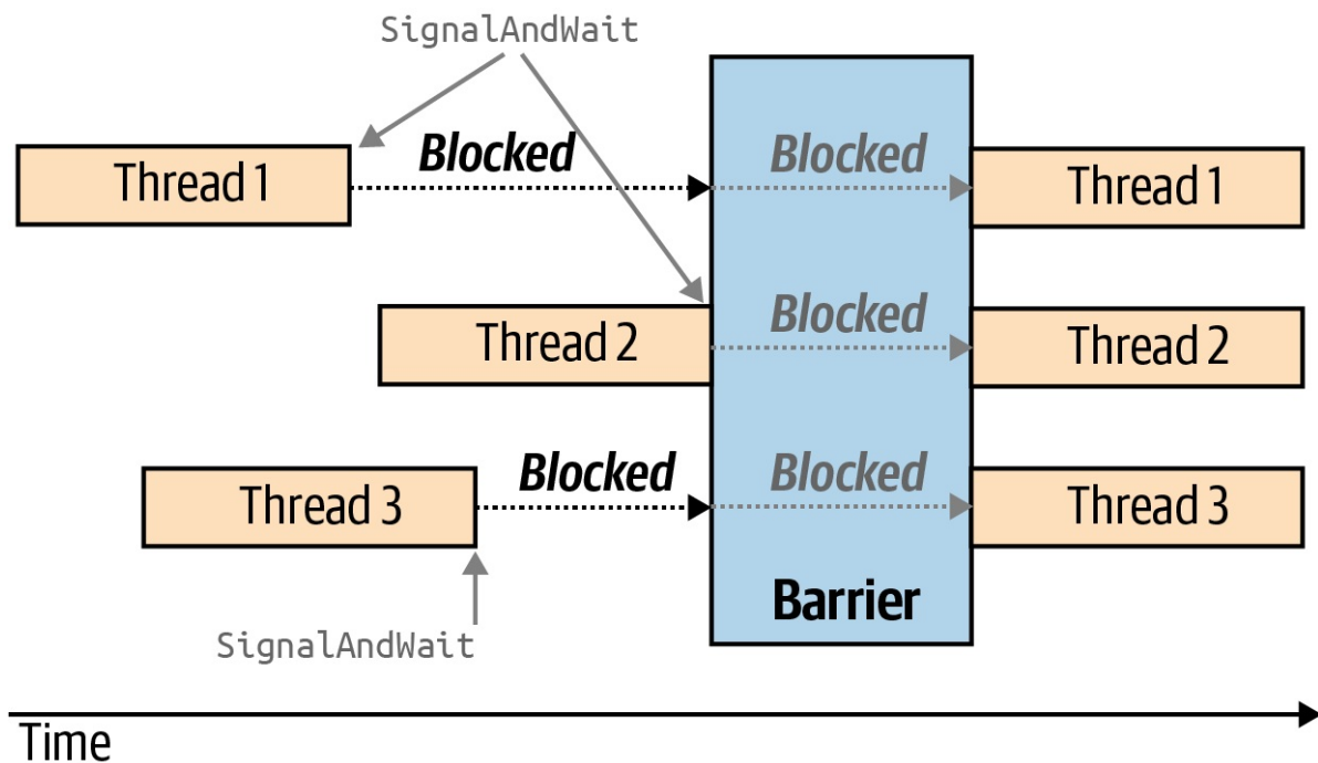
Figure 21-3. Barrier
