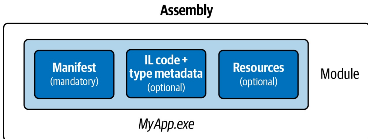
Figure 17-1. Single-file assembly
