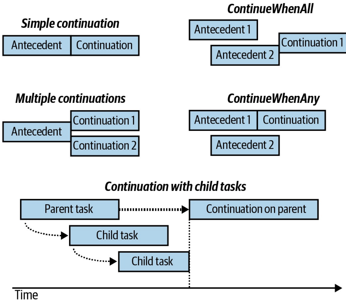
Figure 22-5. Continuations
