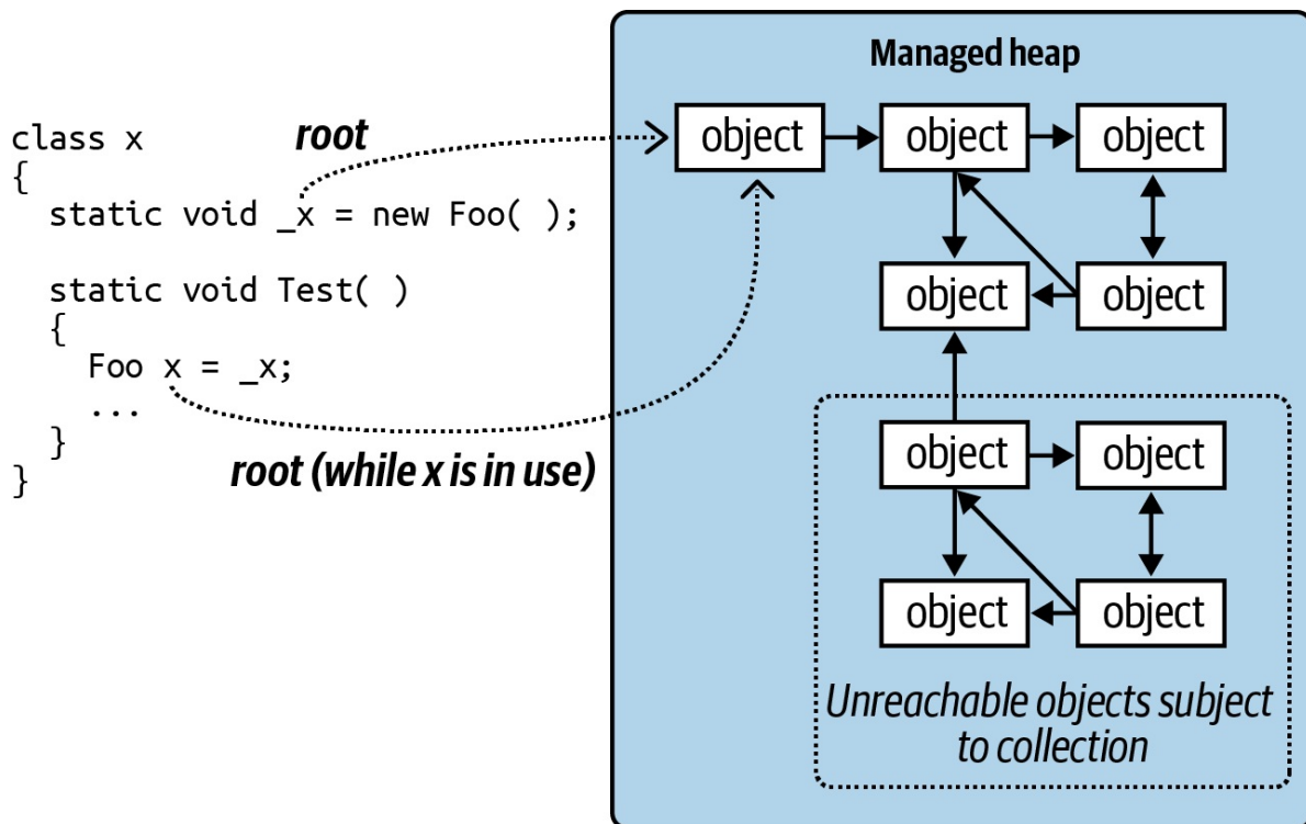
Figure 12-1. Roots
