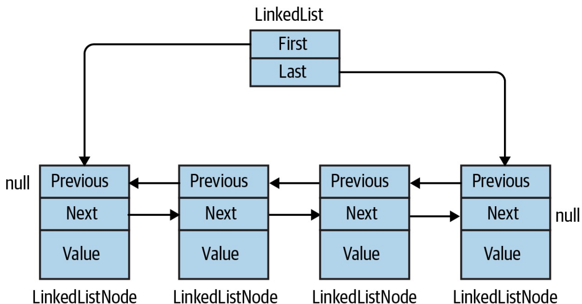
Figure 7-4. LinkedList<T>
