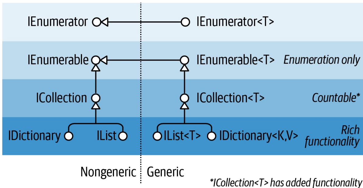
Figure 7-1. Collection interfaces
