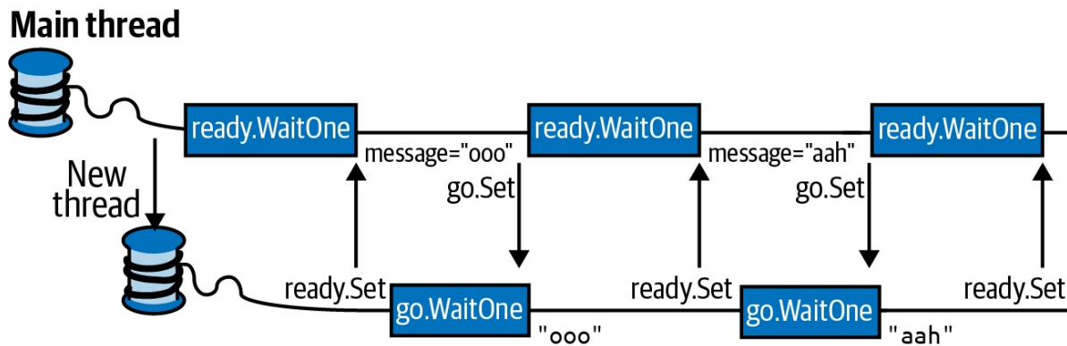
Figure 21-2. Two-way signaling
