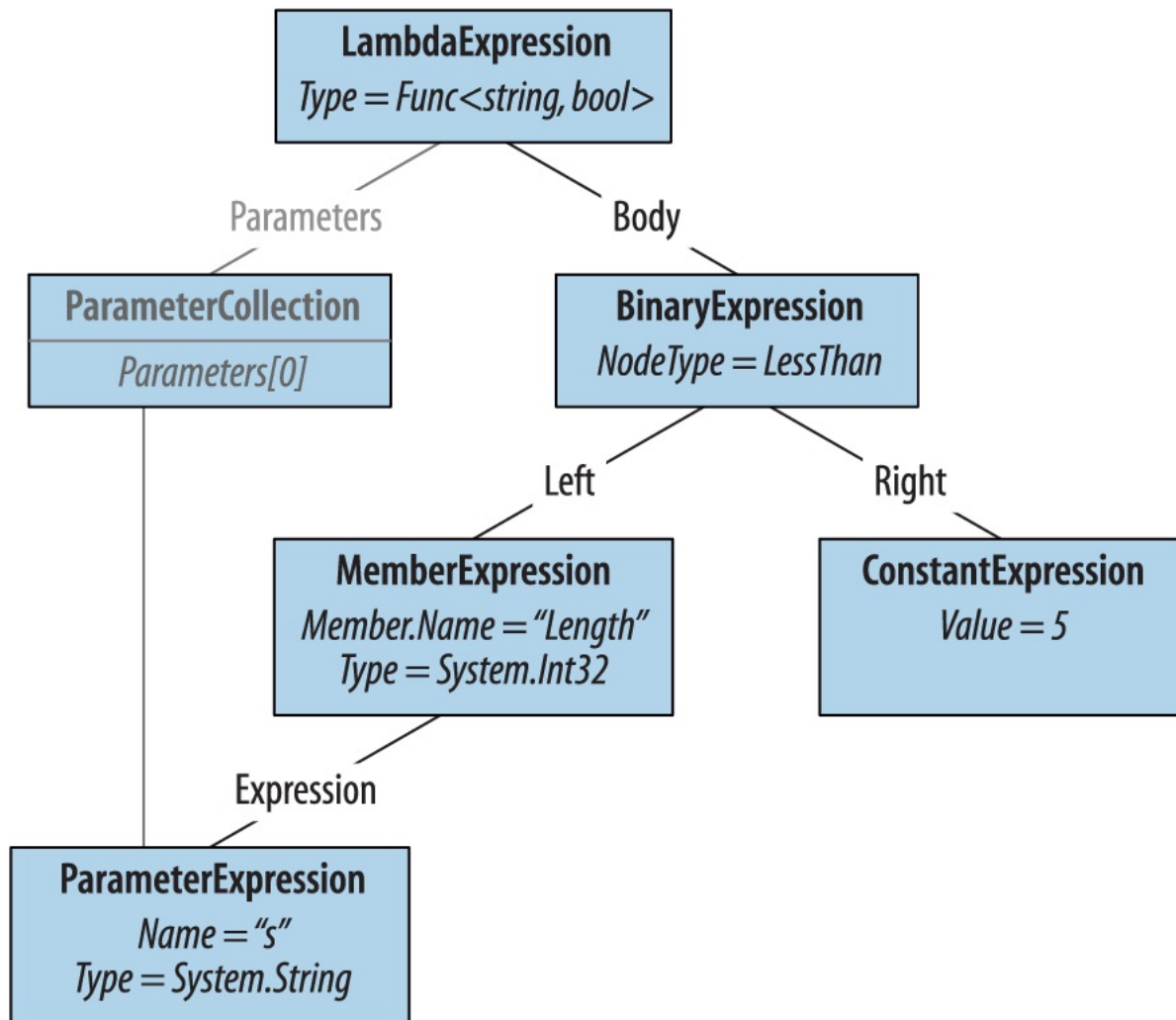
Figure 8-11. Expression tree
