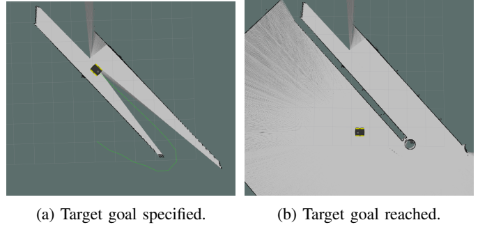
Fig. 10: Simulation validation of the path planning subsystem. (a) visualizes the global path (green) dynamically adjusting to avoid obstacles. (b) depicts the robot successfully arriving at the target pose within the specified tolerance.
