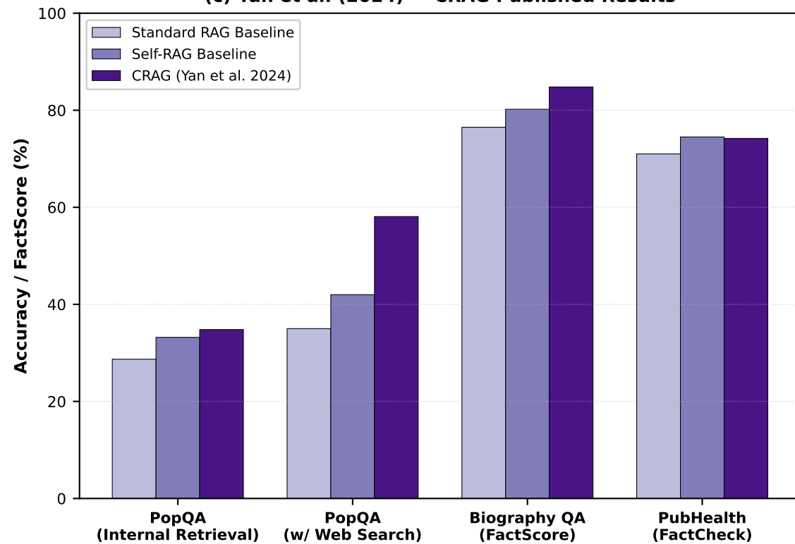
(c) Yan et al. (2024) — CRAG Published Results
