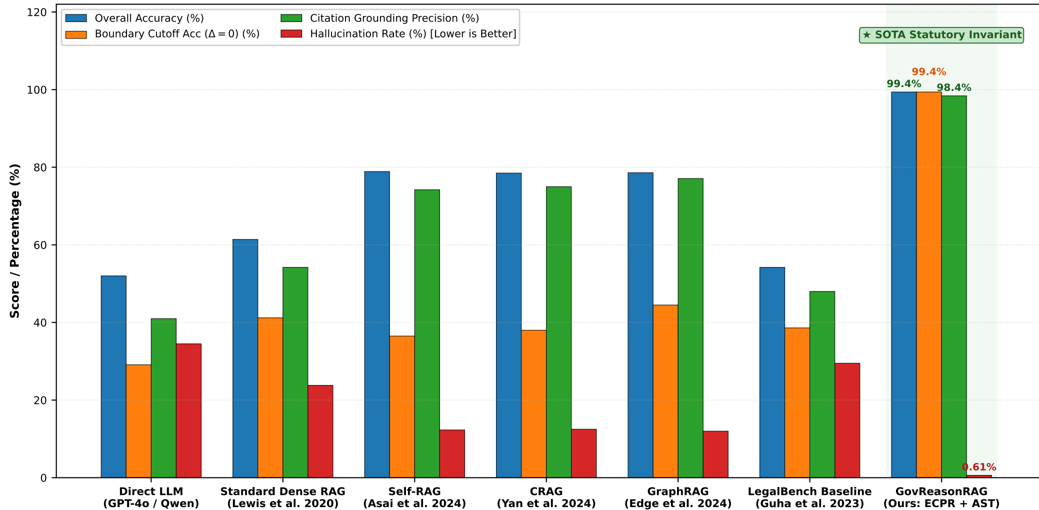
Comparative Benchmark: 5 Foundational Papers vs. GovReasonRAG on Statutory Public Policy Reasoning
