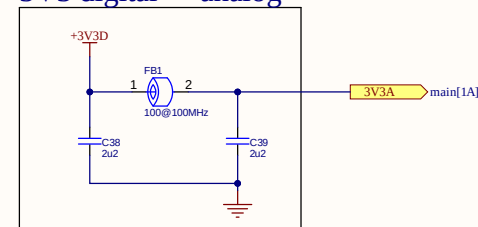
3V3 digital -> analog
