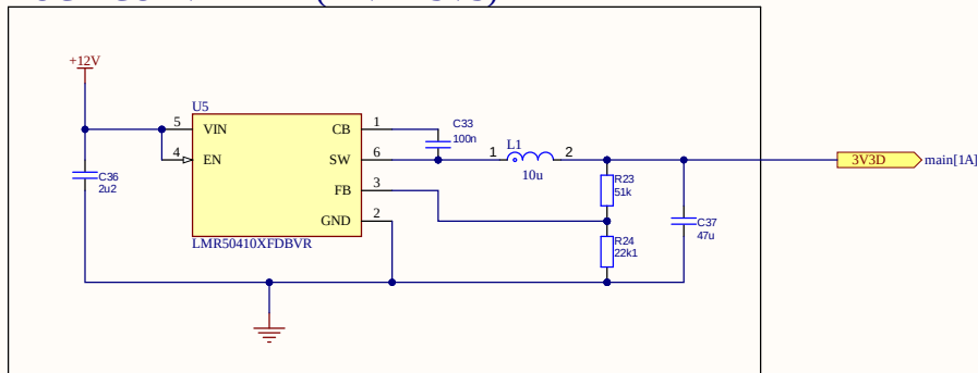
BUCK CONVERTER (12V -> 3V3)
