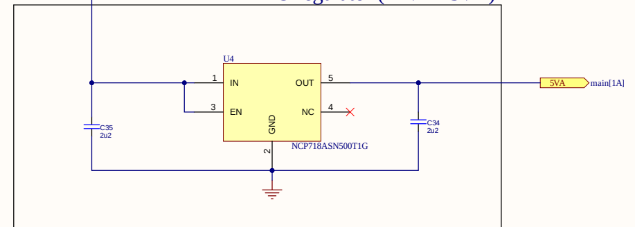
LDO regulator (12V -> 5VA)
