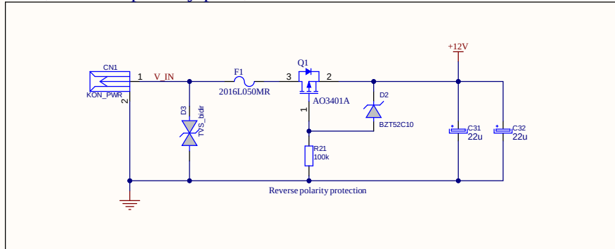
Fuse, Reverse polarity prot., LP Filter
