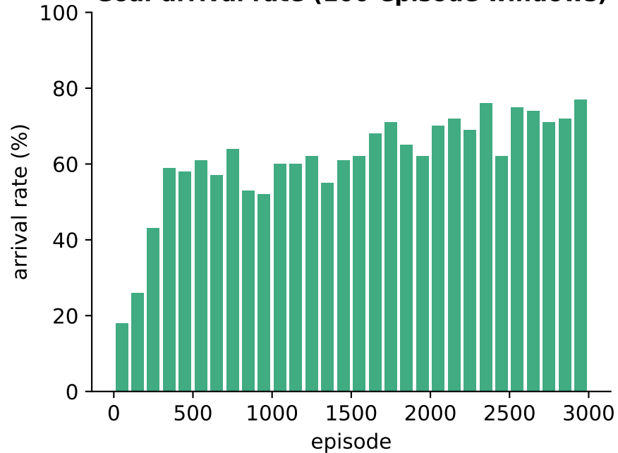
Goal-arrival rate (100-episode windows)
