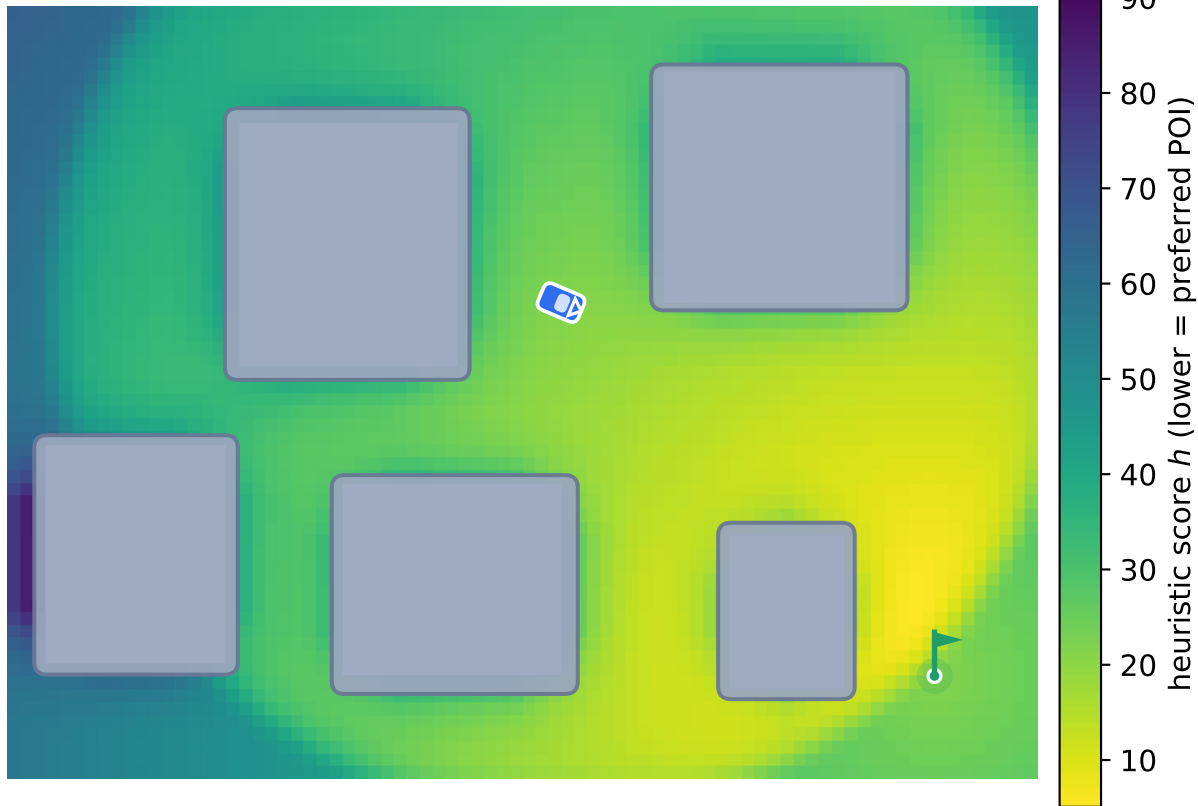
Exploration heuristic over candidate frontier points
