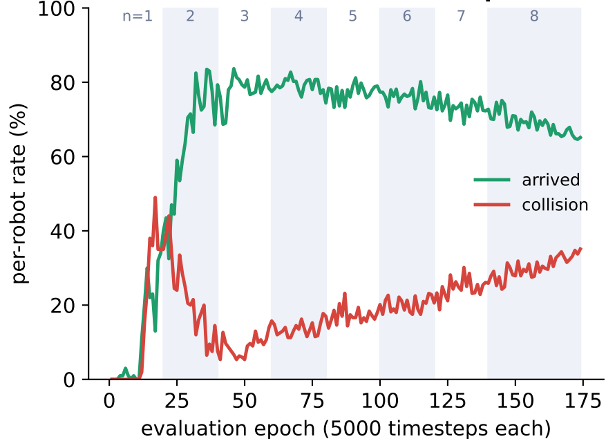
Terminal outcomes (100 eval episodes)
