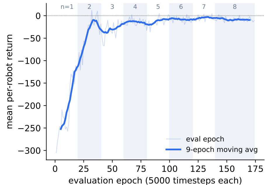
Evaluation return (active robots shaded)
