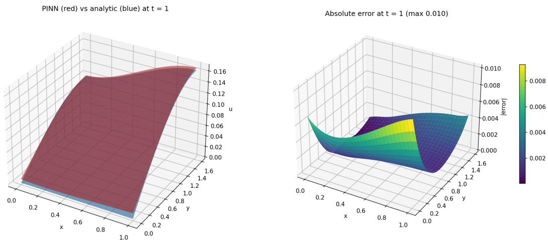
Figure 1: Left: comparison with the analytic solution (blue — analytic, red — numerical). Right: absolute-error field at t = 1 .
