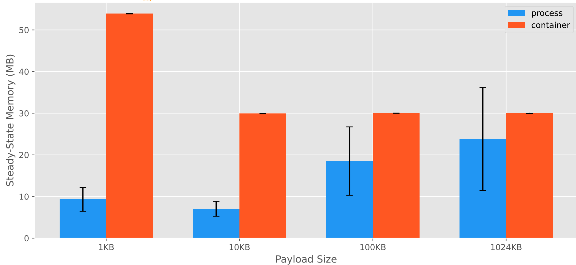
Memory Under Load: Process vs Container — M1 Docker Desktop
