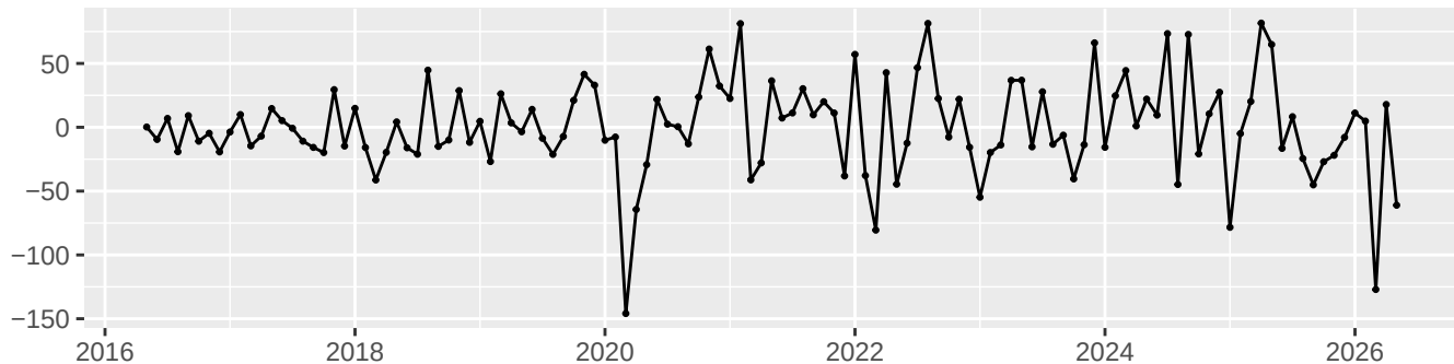
Residuals from ARIMA(0,1,0) with drift
