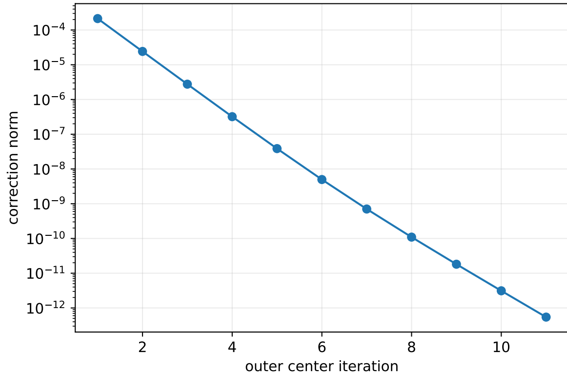
Kretschmann center at R = 0.2M_{\text{tot}}
