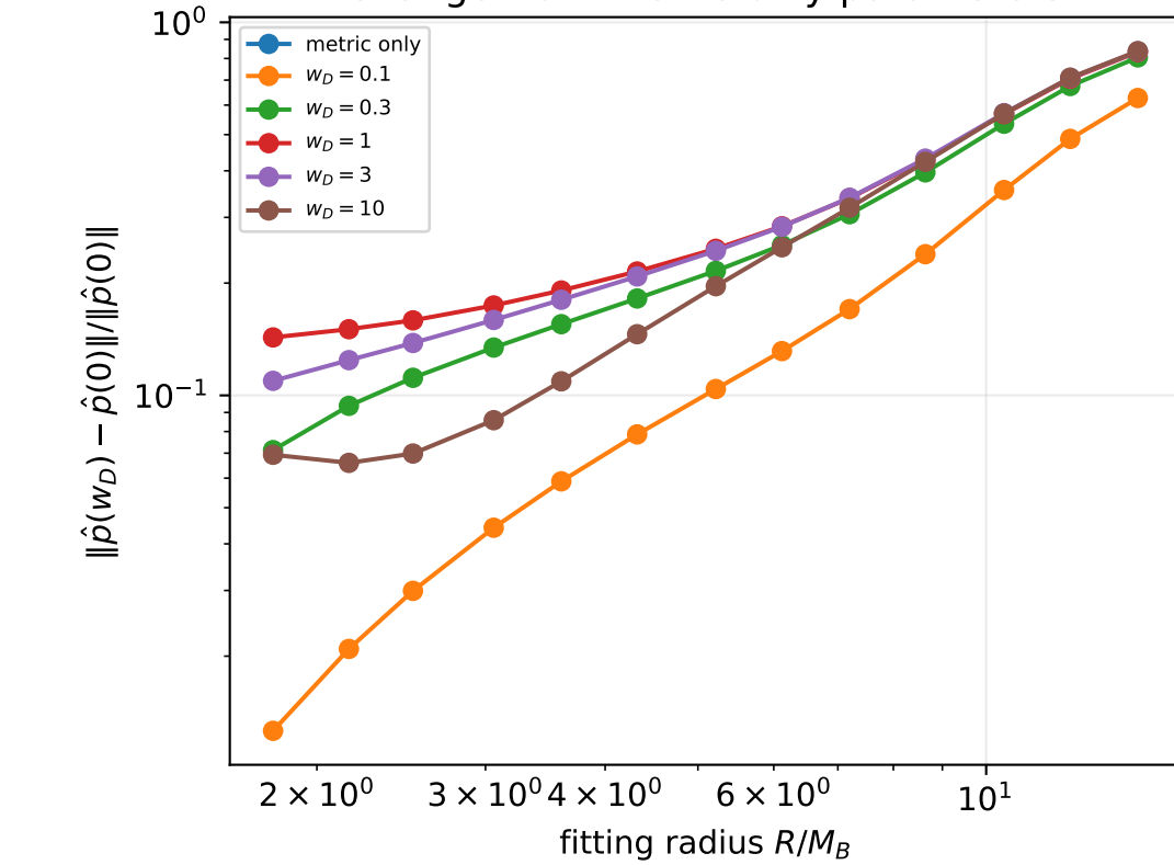
Change from metric-only parameters
