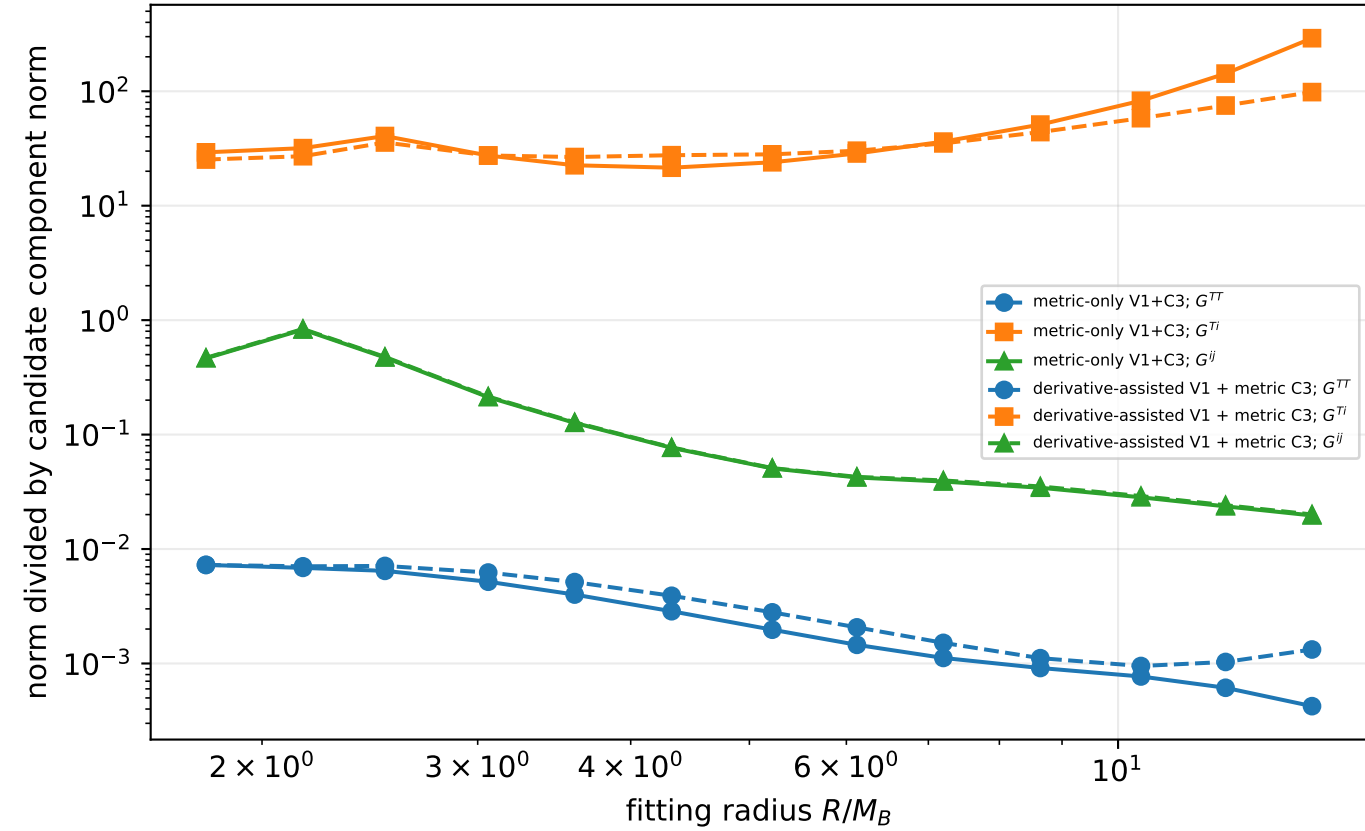
Final surface residual by metric component
