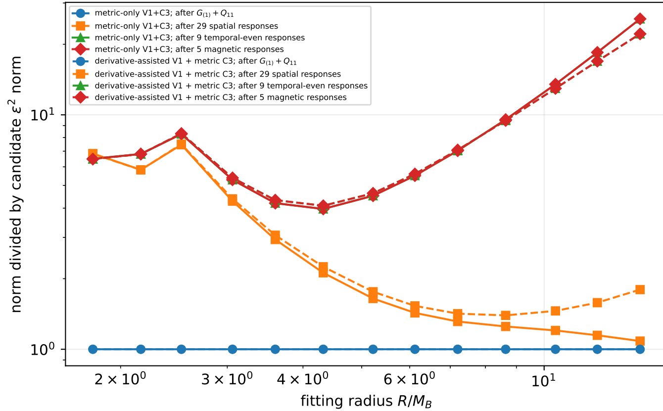
Surface residual after each triangular stage
