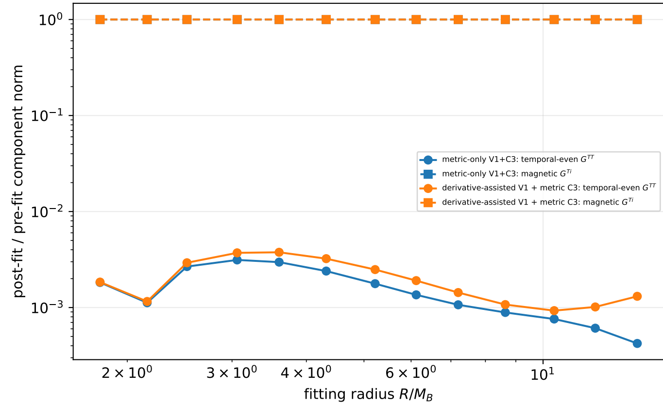
Residual in each newly fitted component block
