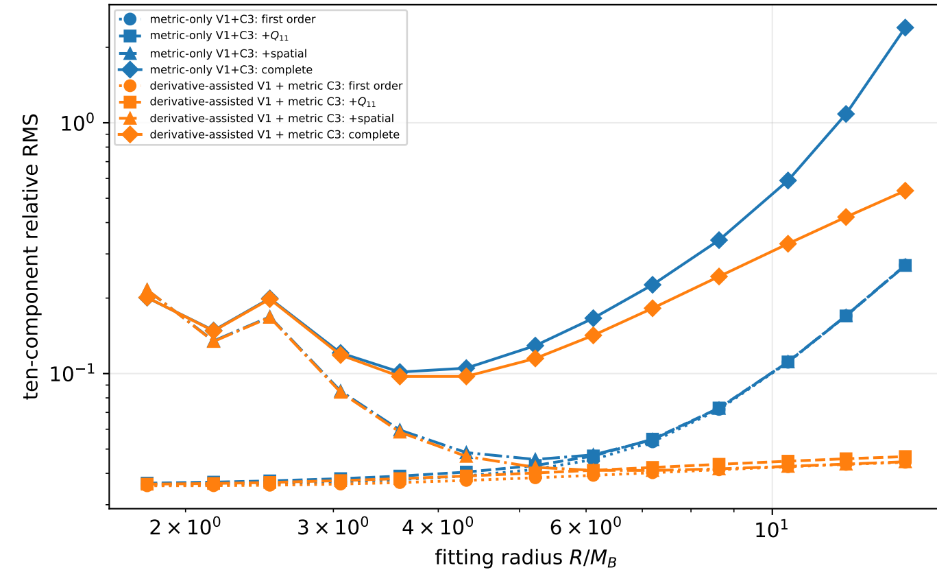
Held-out random interior metric
