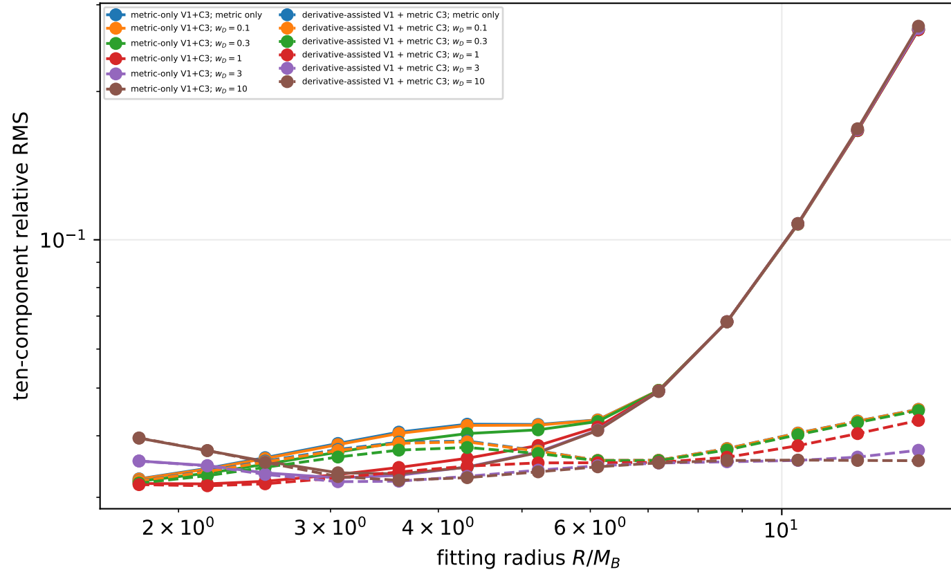
Strain rate + time acceleration: interior metric
