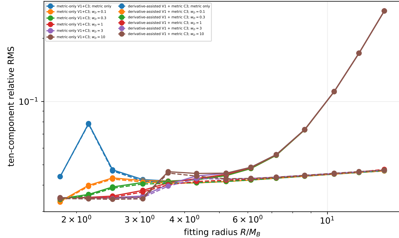
Polar- J = 2 : interior metric
