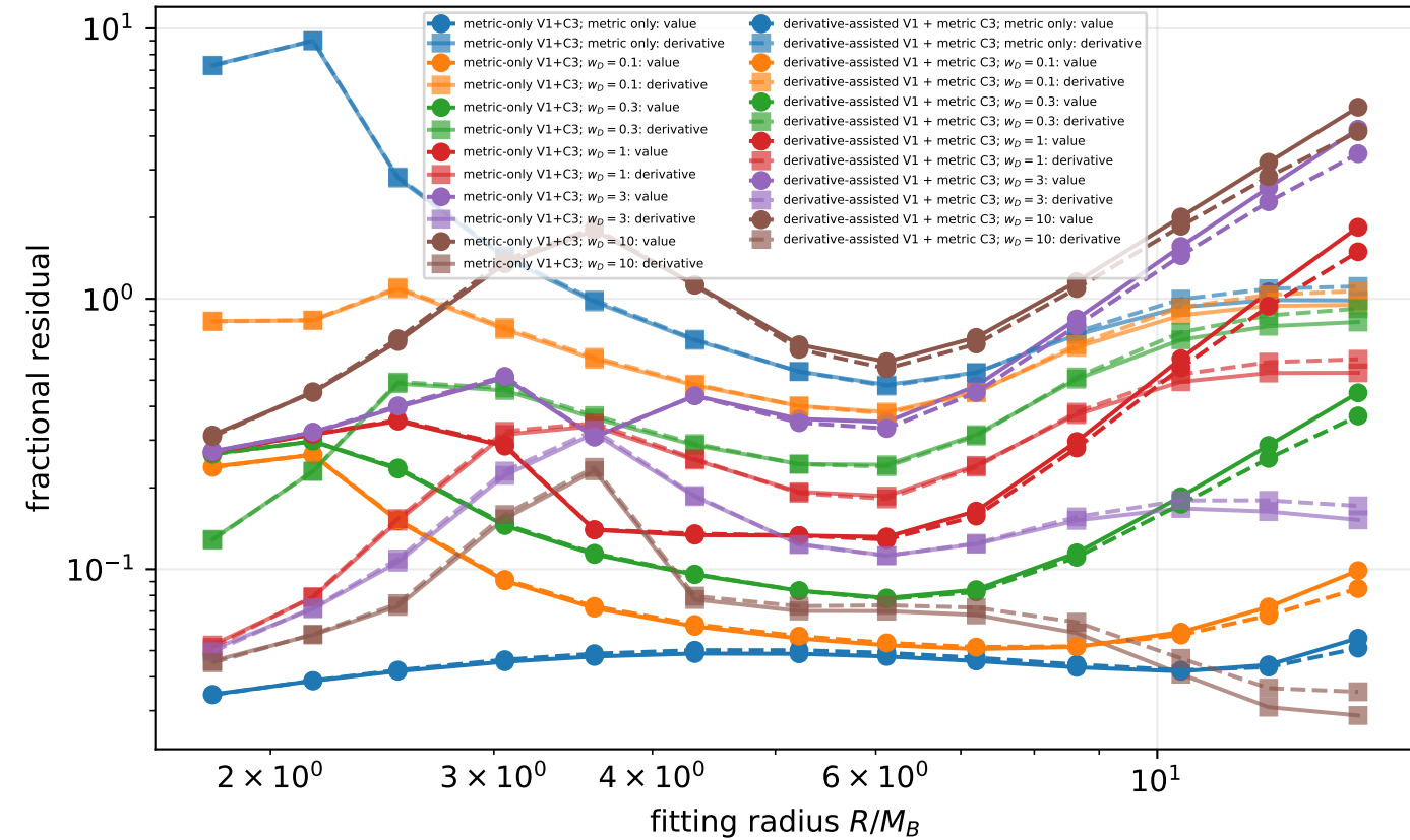
Polar- J = 2 value/derivative residual
