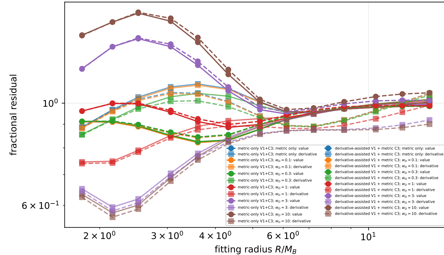
Subset surface value/derivative residual
