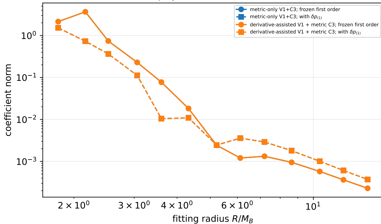
physical electric STF
