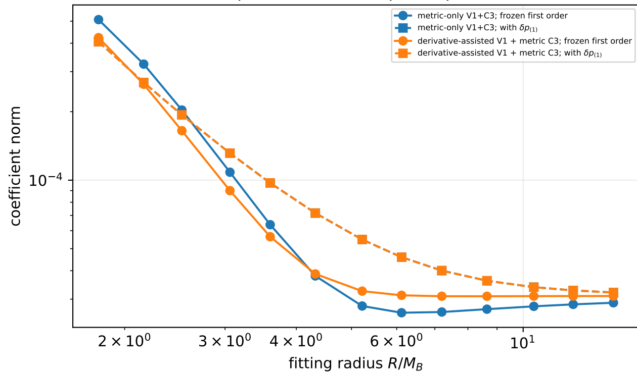
spatial harmonic quadrupole
