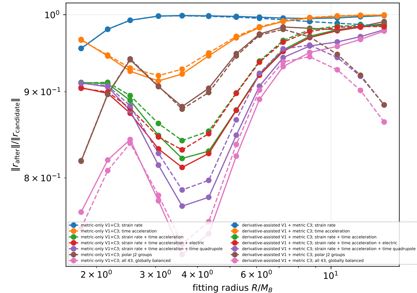
Full surface candidate residual
