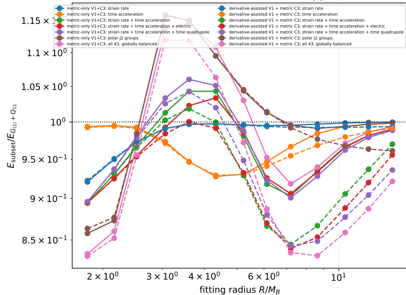
Held-out interior error relative to G_{(1)} + Q_{11}
