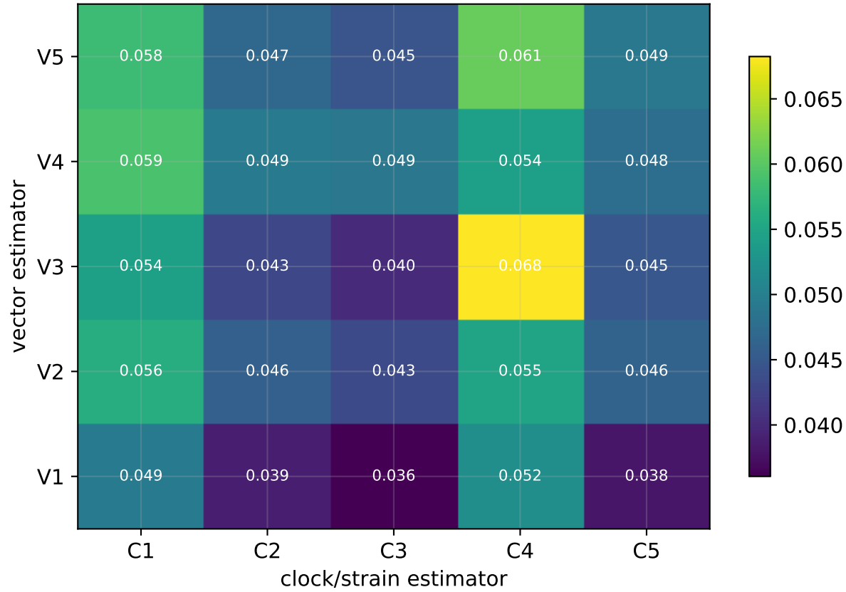
Minimum total RMS over fitting radius
