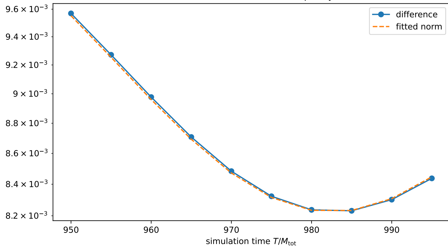
Pointwise strain-rate discrepancy
