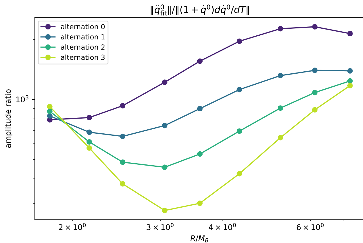
Temporal ODE consistency across worldtube radius (central six observations)
