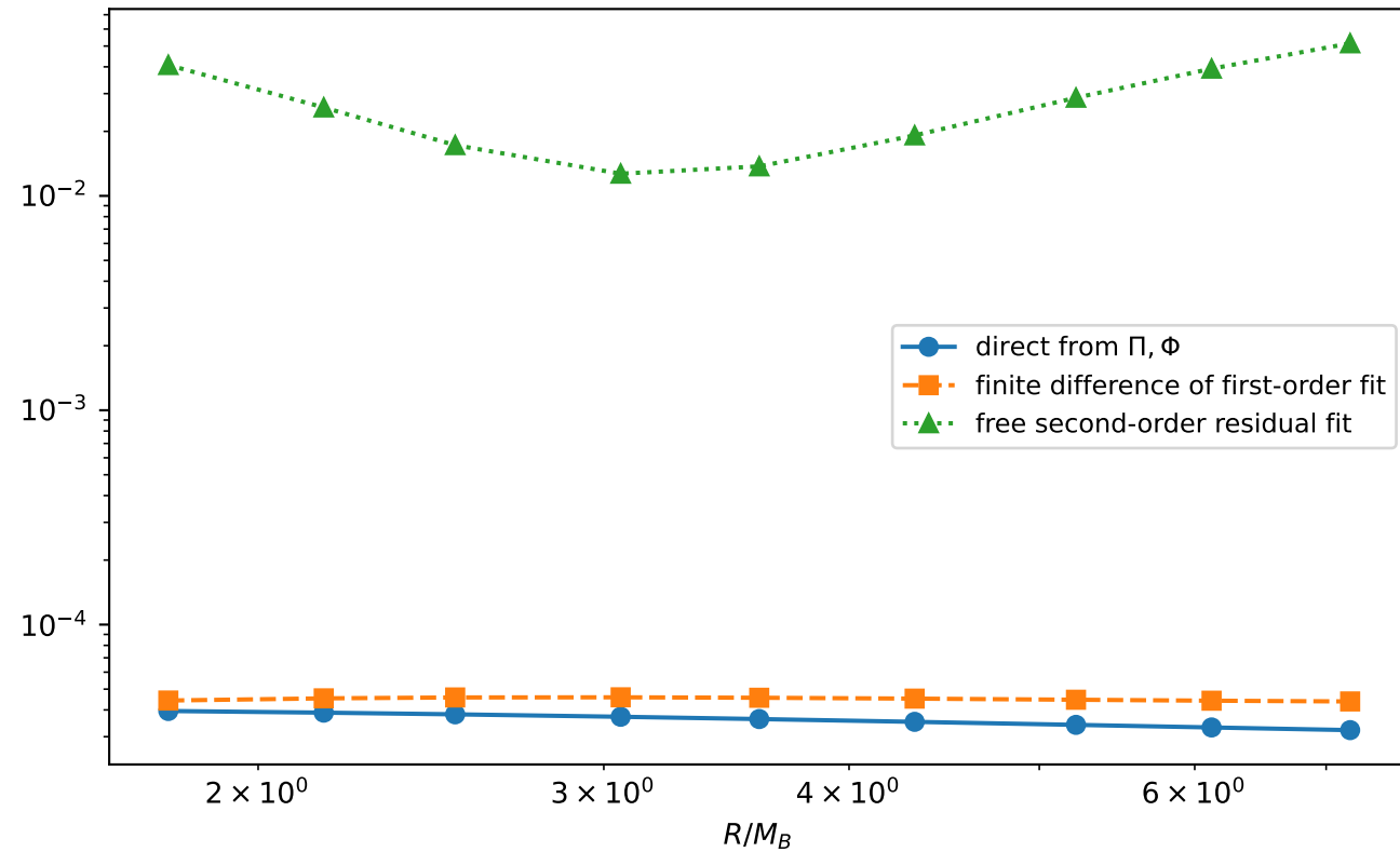
Direct versus finite-difference coefficient rates
