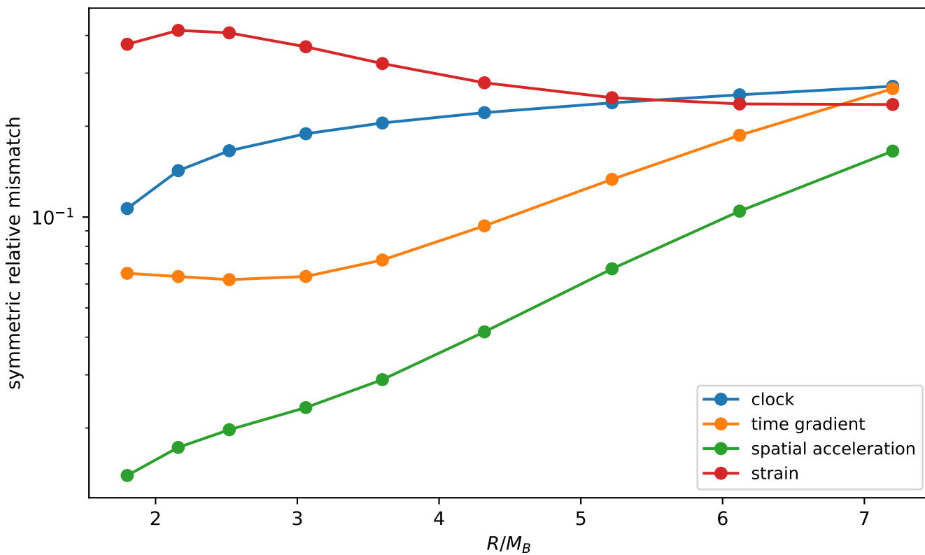
Direct versus finite-difference coefficient rates
