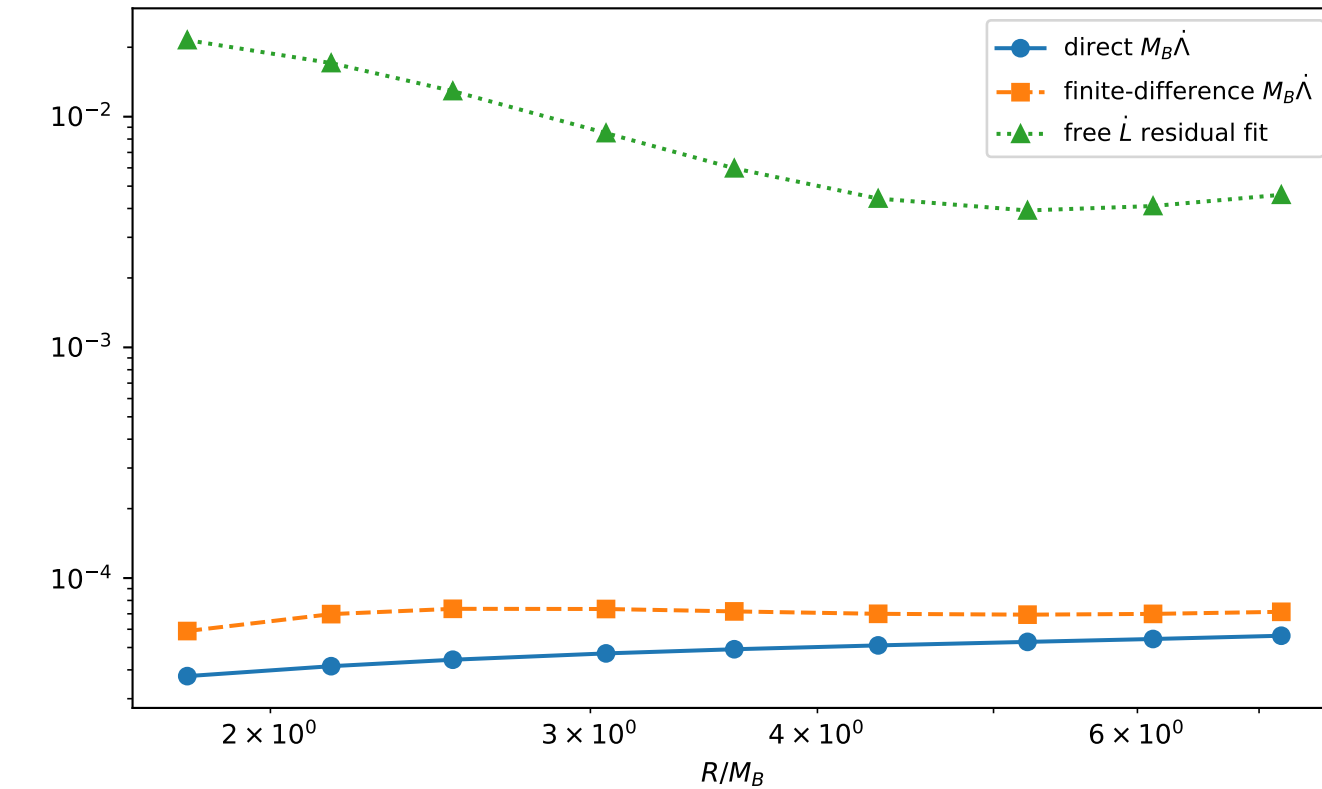
Derivative construction and block closure
