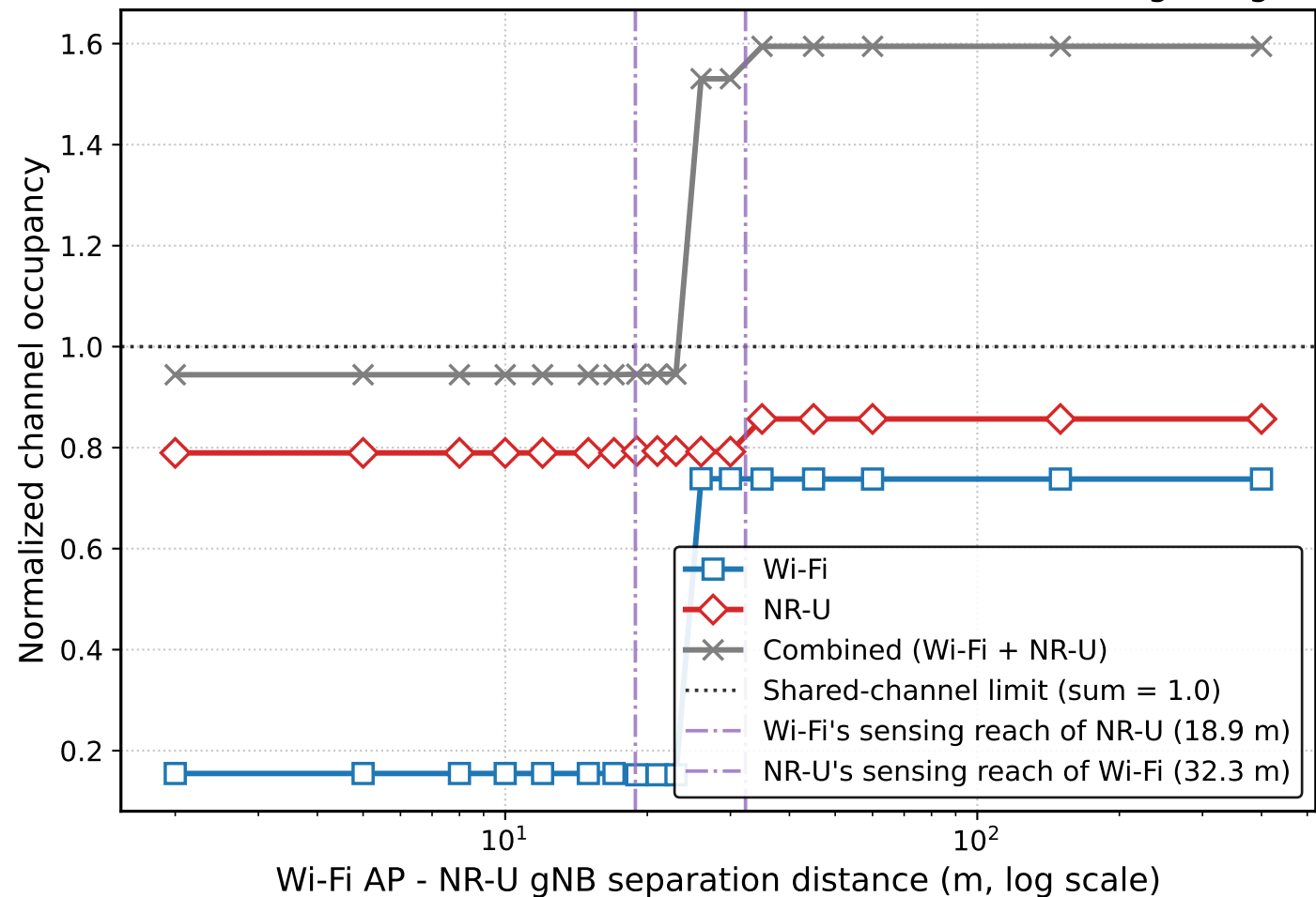
NR-U/Wi-Fi Coexistence: Inside vs. Outside Mutual Sensing Range
