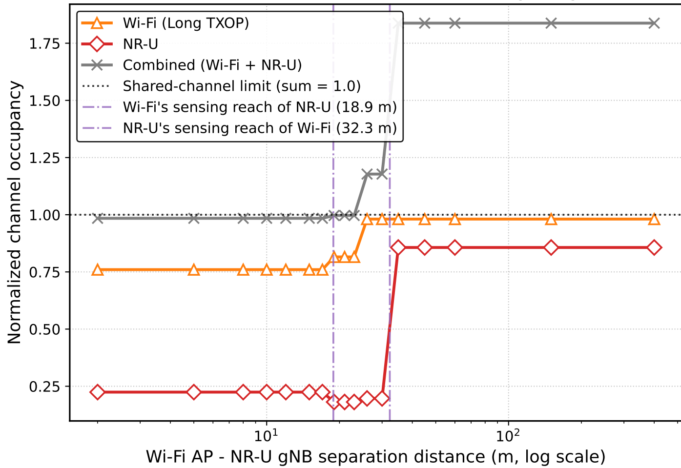
NR-U/Wi-Fi Coexistence: Inside vs. Outside Mutual Sensing Range (Wi-Fi Long TXOP)
