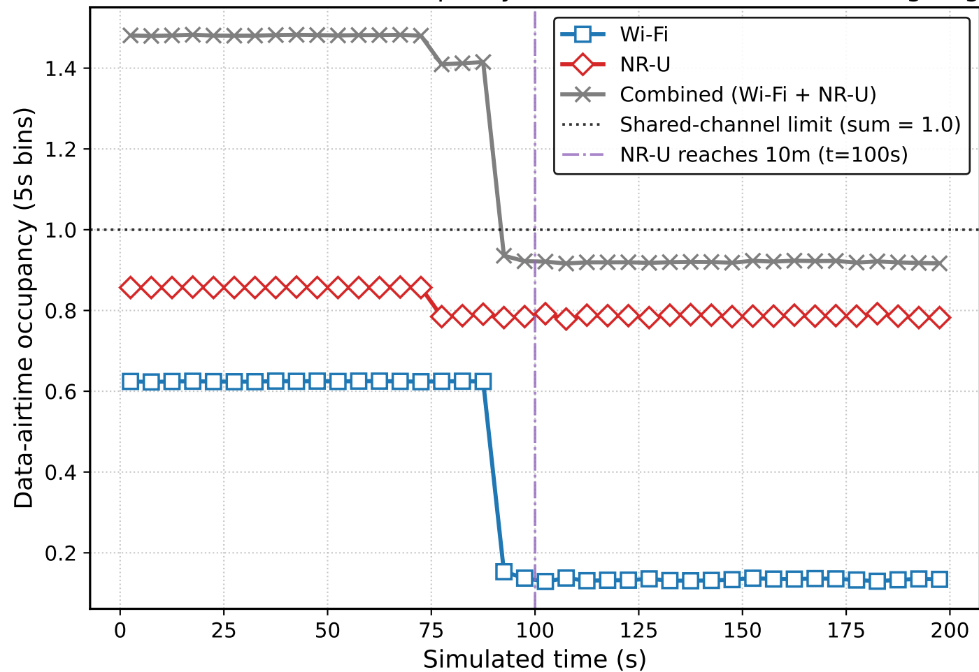
NR-U/Wi-Fi Coexistence: Occupancy as NR-U Enters Wi-Fi's Sensing Region
