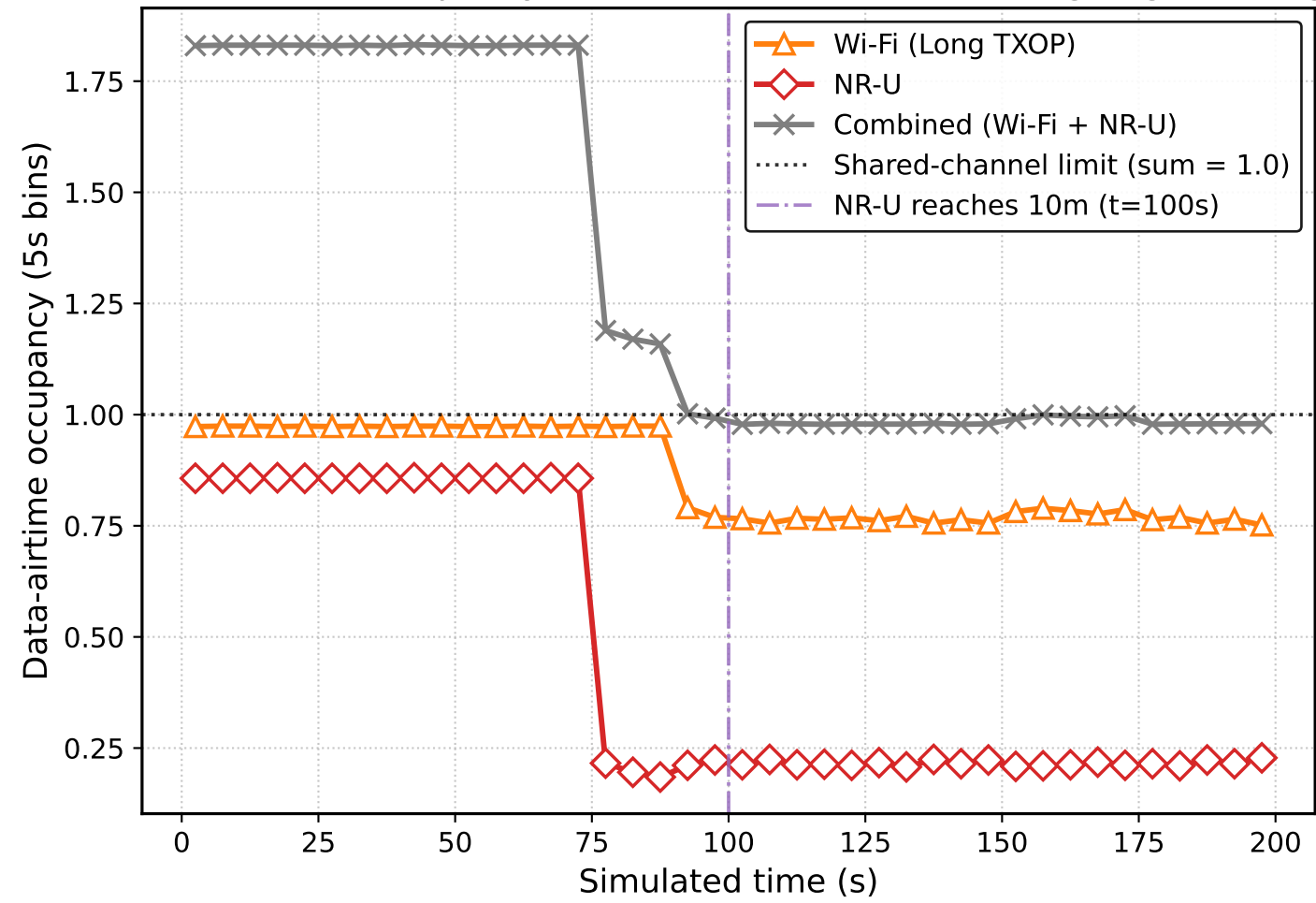
NR-U/Wi-Fi Coexistence: Occupancy as NR-U Enters Wi-Fi's Sensing Region (Long Wi-Fi TXOP)
