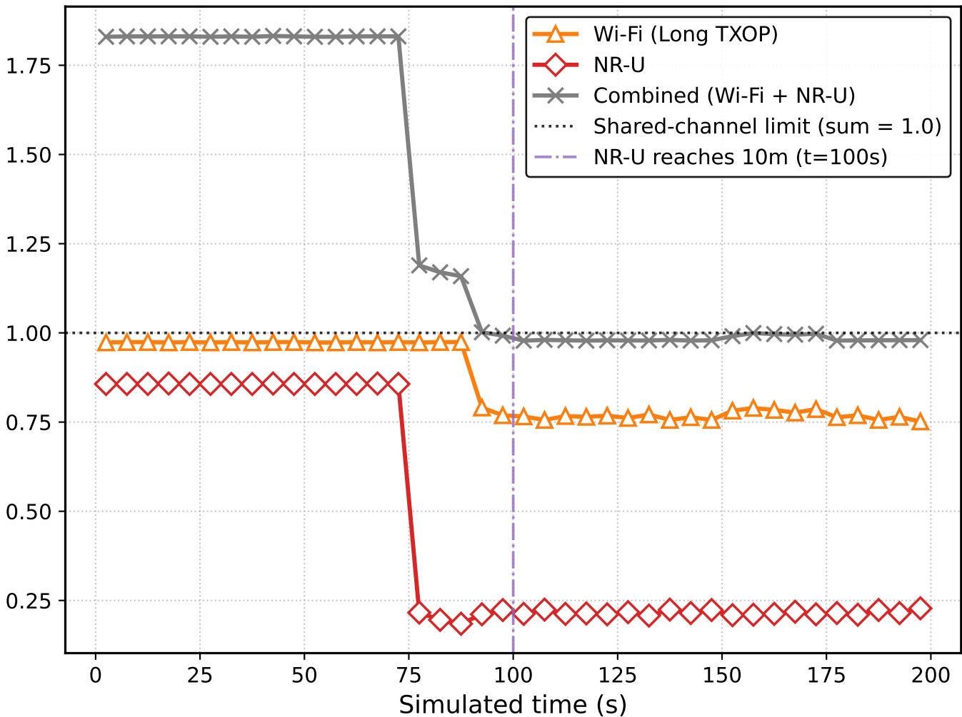
Data-airtime occupancy (5s bins)
