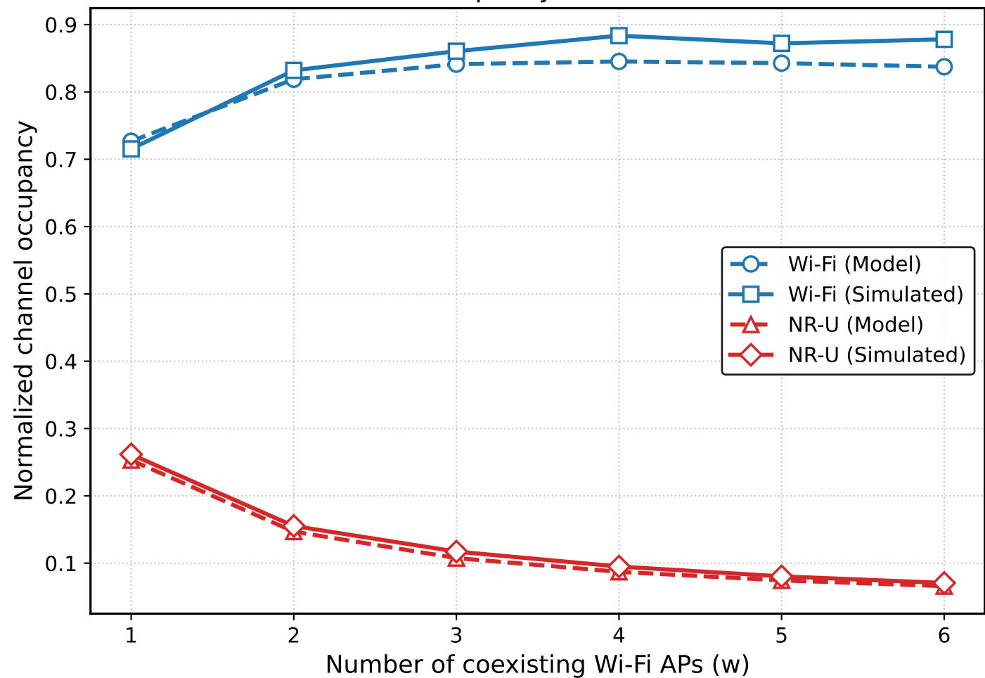
Wi-Fi/NR-U Channel Occupancy: DTMC Model vs. Simulation
