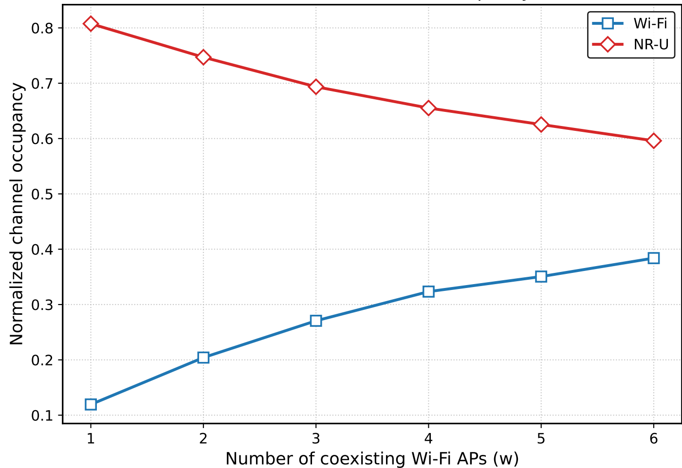
Wi-Fi vs. NR-U: Channel Occupancy
