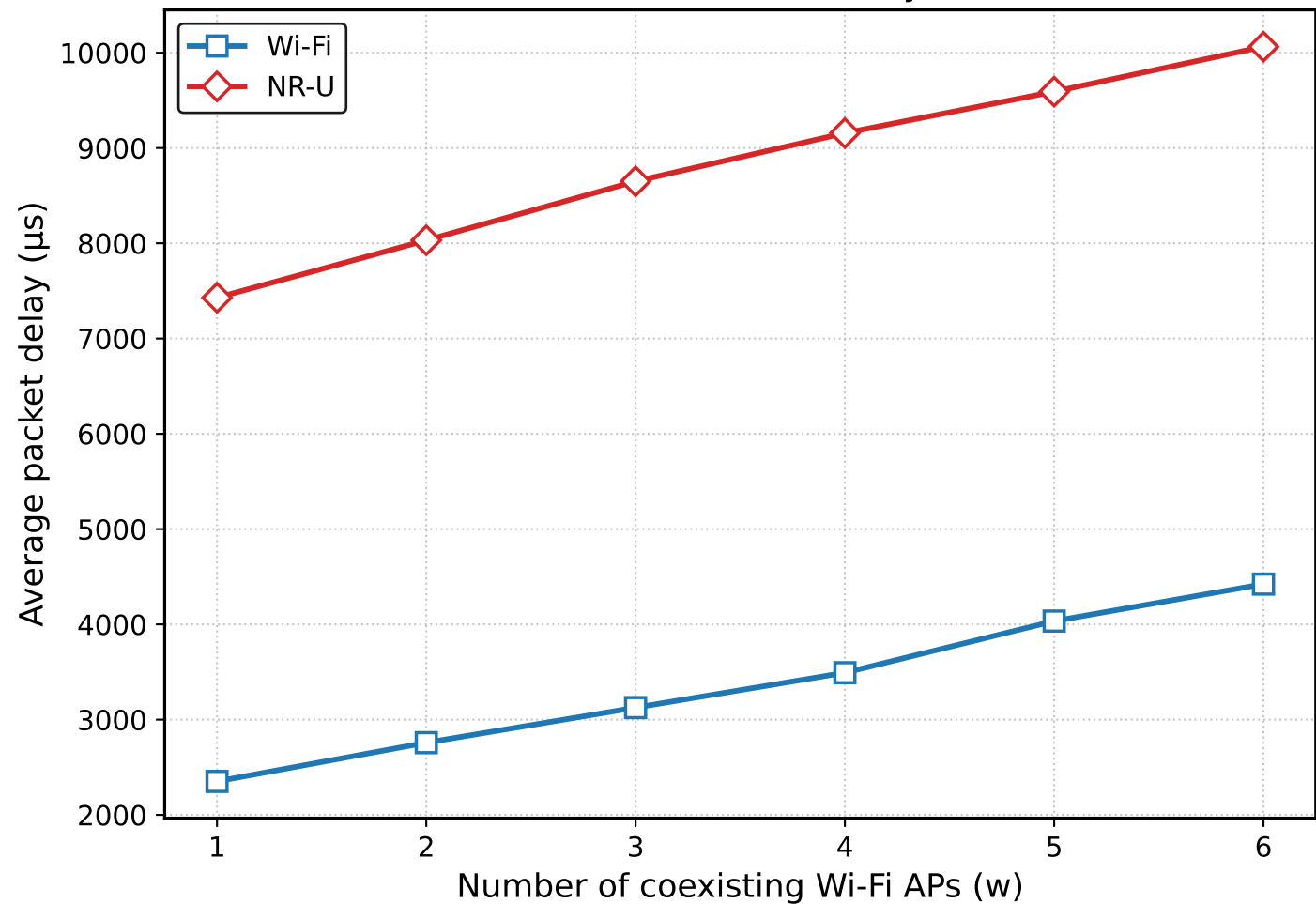
Wi-Fi vs. NR-U: Delay
